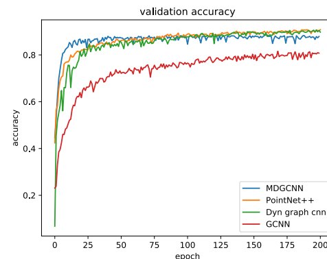
Figure 4.13 – Validation accuracy per epoch on the human body segmentation benchmark introduced in [73] using global 3D coordinates as input.
