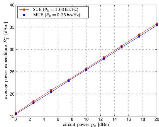
Fig. 12. Average power at the equilibrium as a function of the circuit power. The average power consumption scales linearly with the circuit power in the EE formulation.
