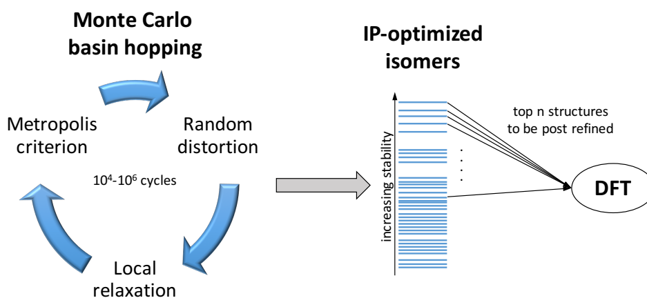
Figure 5.1: Schematic description of the standard basin hopping approach employed in this thesis.
