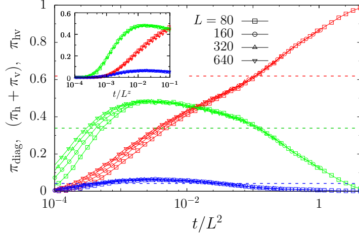
Figure 3.6: The wrapping probabilities for the VM dynamics on a finite square lattice for different values of L , indicated in the keys. We show \pi_{\text{hv}} (red points), \pi_{\text{h}} + \pi_{\text{v}} (green points), and \pi_{\text{diag}} (blue points). The horizontal dashed lines correspond to the exact values of 2d critical percolation wrapping probabilities \pi_{\text{hv}}^{(p)} , \pi_{\text{h}}^{(p)} + \pi_{\text{v}}^{(p)} and \pi_{\text{diag}}^{(p)} , for a lattice with unit aspect ratio, see Sec. 1.3. In the main plots, the wrapping probabilities are plotted against t/L^2 . In the inset, the same data are plotted against the rescaled time t/L^z , with z \simeq 1.67 .
