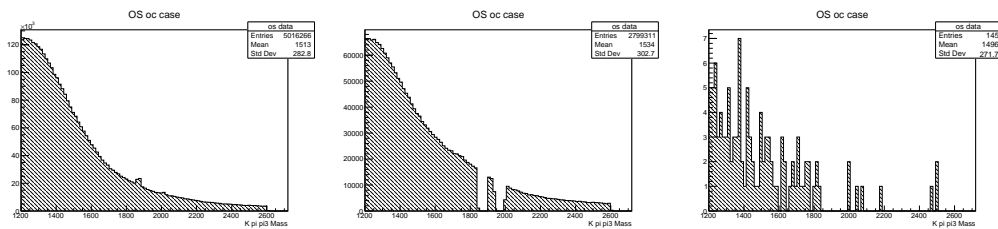
Figure 4.32: Invariant mass of the K^{*0}\pi_3 system, with trigger, stripping and fiducial cuts applied: on the left without veto and on the middle with the veto. The plot on the right is after the full selection. OC case
