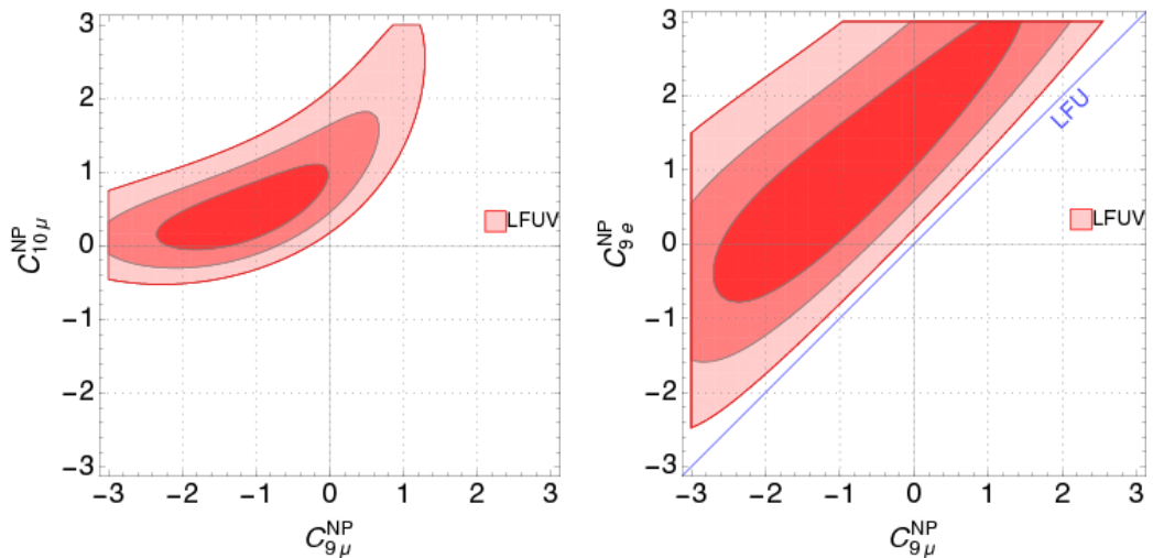
Figure 1.6: Phenomenological fits on the LU observables assuming new physics only in muons and only in C_9 and C_{10} (left) or only in C_9 but for electrons as well (right). 1, 2 and 3\sigma contours are shown. On the right figure, the LFU line is also shown. Figures taken from Ref. [34].
