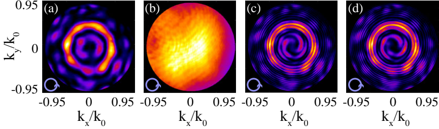
Figure 5.15: Raw experimental data. (a) Fourier image of the far field intensity radiated in left handed circular polarization (LHCP) by a cavity of radius 2 \mu\text{m} , dressed by N = 19 pairs of antennas for the V-type structure, at resonance for a WGM m = 22 at \lambda = 772.5 \text{ nm} . (b) Fourier image of the intensity (in LHCP) of the reference beam used for interferometric phase retrieval. (c-d) Interferograms obtained when combining reference and analysed beam (for two different phase delays). We see a spiral with two arms which confirms the generation of a beam of OAM \ell = m - N - 1 for LHCP.
