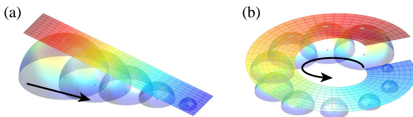
Figure 5.2: Scattering of a wave propagating along arrays of point scatterer according to the Huygens principle. (a) Case of a linear array: each point scatters spherical wavefronts, which are delayed in time relative to each other due to the finite propagation speed of the incident wave. This scattering is equivalent to diffraction by a grating as the coherent sum of individual wavefronts in the far-field approximates to a tilted plane wave. (b) Case of an azimuthal array: the description is similar to the linear case except that the coherent sum is now a helical wave.
