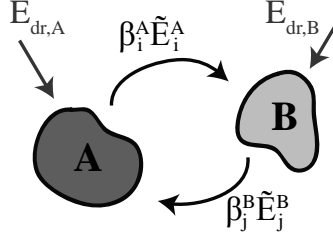
Figure 3.4: Sketch of the bidirectional interaction between two resonators described QNM. The resonators are driven by an external source and they scatter onto each other a field proportional to a superposition normalized QNMs (here we only indicate QNM i for A and j for B ).
