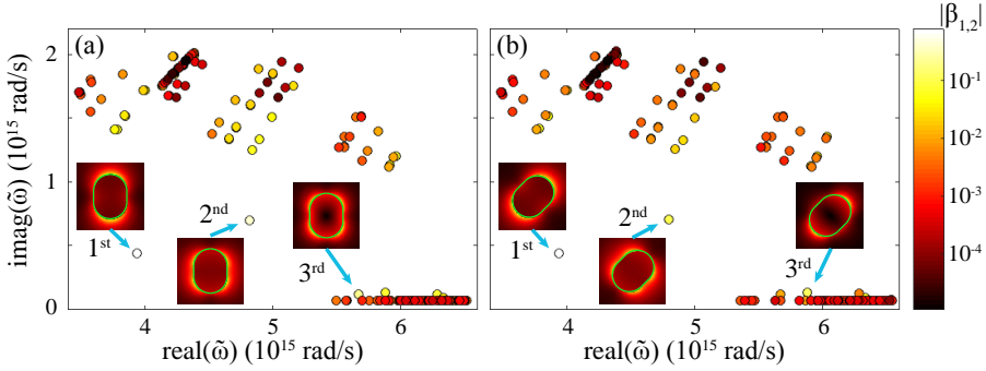
Figure 3.15: Relative contribution of the QNMs of nanorods 1 and 2 in the reconstruction of the dimer bright mode. (a) and (b) show the position in the complex frequency plane of the 200 QNMs used to describe nanorod 1 and nanorod 2 in the coupled QNM theory. The two nanorods should theoretically have exactly the same QNM, and we indeed observe that the first 200 QNMs of rod 1 and rod 2 have the same complex resonance frequencies. Each point is colour coded (in logarithmic scale) with respect to the magnitude of the coefficient \beta_{i,m} describing the contribution of mode m of nanorod i in the reconstruction of the bright mode of the dimer. The insets show the mode profiles of the first three most important modes in the reconstruction. The most important mode of rod 1 and 2 is, as expected, the long axis dipolar mode.
