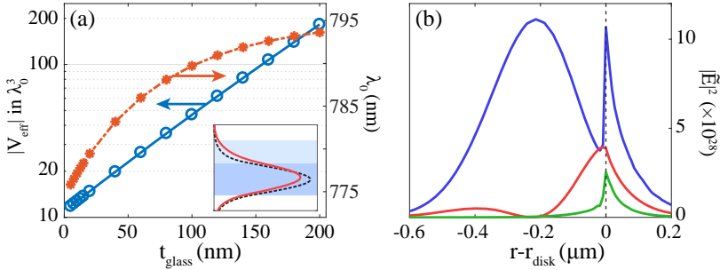
Figure 5.11: Mode volume and normalized electric field at the glass-air interface of a microdisk cavity (radius 2 \mu\text{m} , t_{\text{Si}_3\text{N}_4} = 200 \text{ nm} , mode m = 22 ). (a) Effective mode volume (in unit of wavelength) at the maximum of the field at glass-air interface (solid blue), and resonance wavelength (dashed orange) as a function of top glass layer thickness. The mode volume exponentially increases as we increase the glass layer thickness ( n = 1.5 ) as the glass-air interface is moving away from the \text{Si}_3\text{N}_4 where the field remains confined. The inset shows in dashed black the normalized field intensity of the mode for the symmetric \text{Si}_3\text{N}_4 cavity ( t_{\text{glass}} = 0 ) and in red for t_{\text{glass}} = 150 \text{ nm} . Since away for the core the mode field is decreasing exponentially, the mode is feeling less and less the perturbation by additional glass thickness and therefore the resonance wavelength converges towards \approx 795 \text{ nm} . (b) Normalized intensity of the 3 components of the cavity electric field m = 22 at the glass-air interface for t_{\text{glass}} = 150 \text{ nm} : blue is |\vec{E}_r|^2 , red |\vec{E}_{\text{phi}}|^2 and green is |\vec{E}_z|^2 . We note that 230 \text{ nm} from the edge of the disk, the field is maximal on its radial component and minimal on the other two.
