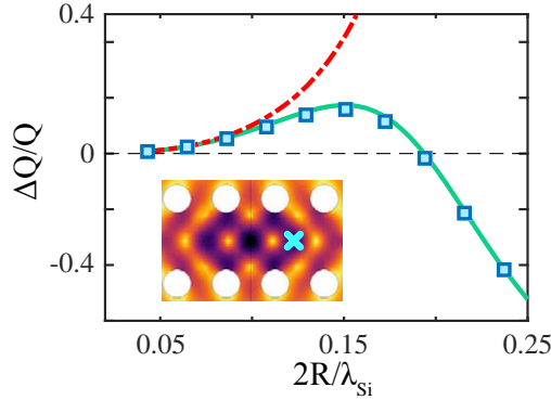
Figure 2.5: Broadening and narrowing of the resonance as a function of the size of an air sphere perturbation in the median plane of the PhC slab, at a fixed position x = 360 nm (indicated by a blue cross in the caption of the mode profile). Blue squares are calculations from COMSOL, red dashed line is Eq.(2.2) with the static polarizability \alpha , and green solid line is with the dressed polarizability \alpha_d .
