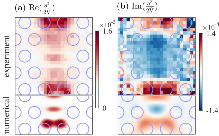
Figure 2.6: Maps of (a) \text{Re} \tilde{V}^{-1} and (b) \text{Im} \tilde{V}^{-1} computed with the QNM-solver 30 nm above the semiconductor membrane (bottom) and directly inferred from the \Delta\tilde{\omega} measurements using Eq.(2.2) with a tip polarizability \alpha_{\text{tip}} = 166\alpha_0 (top). Note that the experimental values are all rescaled by a factor 1/4.
