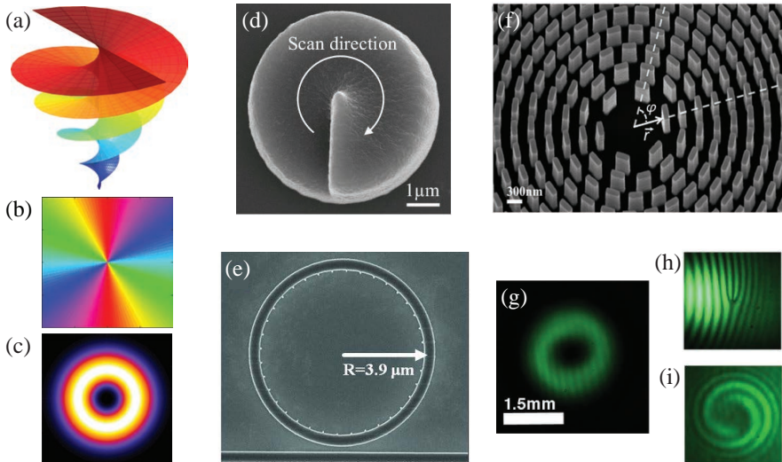
Figure 5.1: Orbital angular momentum (OAM) of light: concept and generation. (a) Helical wavefront carrying an OAM of +2. (b-c) Resp. transverse phase and intensity profiles of a Laguerre-Gaussian beam carrying an OAM of +2. (d) Scanning electron microscopy (SEM) image of a 5 \mu\text{m} diameter spiral phase plate. Reprinted from [217]. (e) SEM image of a microring resonator with angular grating patterned along the inner wall. Reprinted from [218]. (f) SEM image of a Q-plate metasurface, reprinted from [219]. (g-i) Typical measurements of OAM beams (here carrying an OAM -2), showing an intensity profile transverse to the beam with a null in its center (g), and interferograms obtained with a tilted plane wave reference beam (pitchfork dislocation, (h) and a spherical phasefront reference (spirals (i)) [219].
