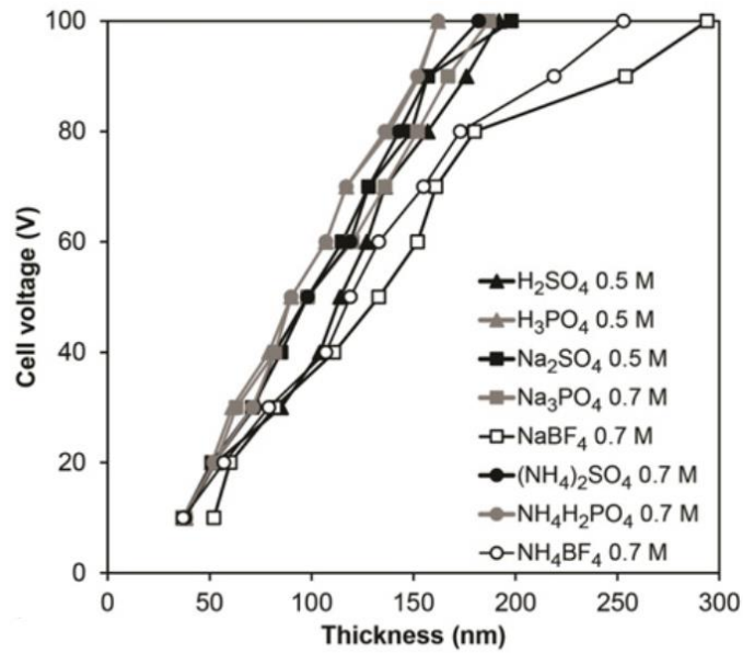
Figure 47: Oxide layer thickness of ASTM Grade 2 titanium samples anodized at a current density of 20mA/cm 2 in different electrolytic solutions as a function of the cell potential for different electrolytes (from [68]).
