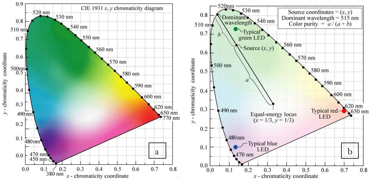
Figure 4: CIE xy chromaticity diagram (a) and chromaticity diagram showing the determination of the dominant wavelength and color purity using the equal-energy locus ( x = 1/3, y = 1/3 ) as the white reference (b) (from [31]).
