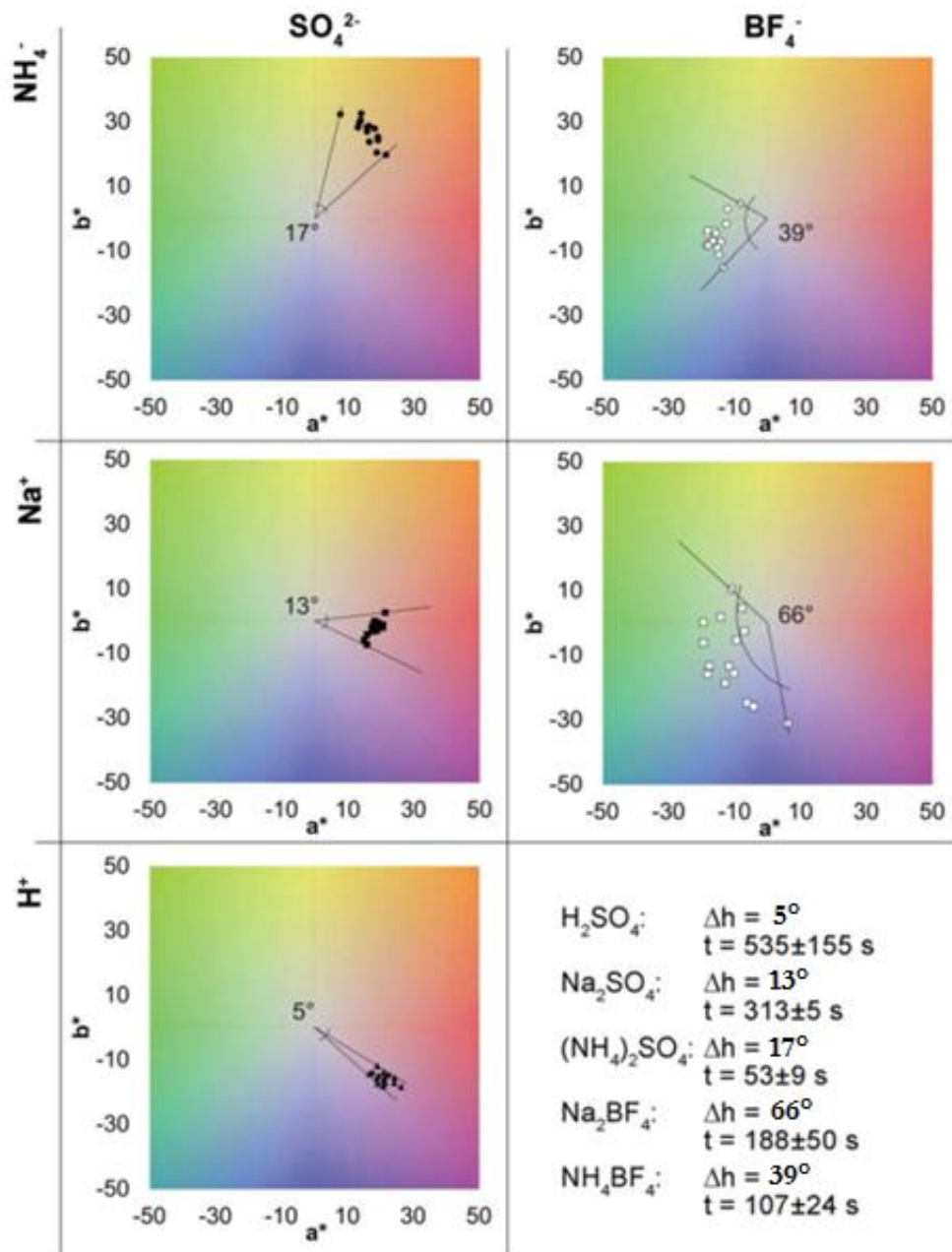
Figure 49: Color coordinates in an a^* - b^* plane of 15 replicates of ASTM grade 2 titanium samples anodized at 100 V at a current density of 20 mA/cm 2 in different electrolytes. The angular value reported in the graphs corresponds for each solution to the maximum hue variations between all the samples series. Anodizing times and their standard deviation are also reported on the right of the figure (from [68]).
