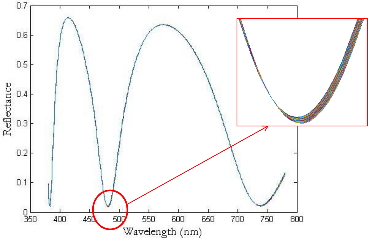
Figure 113: Reflectance spectra for observation angles ranging from 44.3° to 45.7° of a modeled anodized titanium sample with an oxide layer thickness of 180 nm and refractive indexes extracted from [72]. On the right is presented a magnification of the area around the second minimum.
