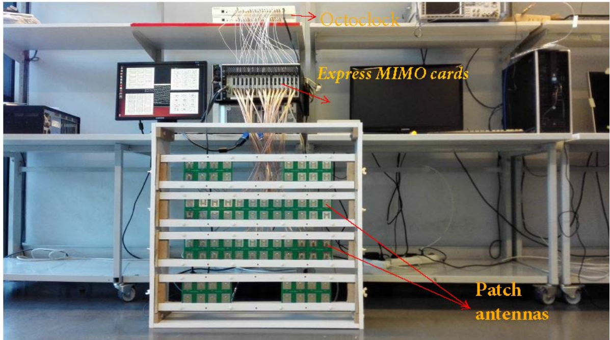
Figure 6.1: Eurecom MaMIMO prototype
