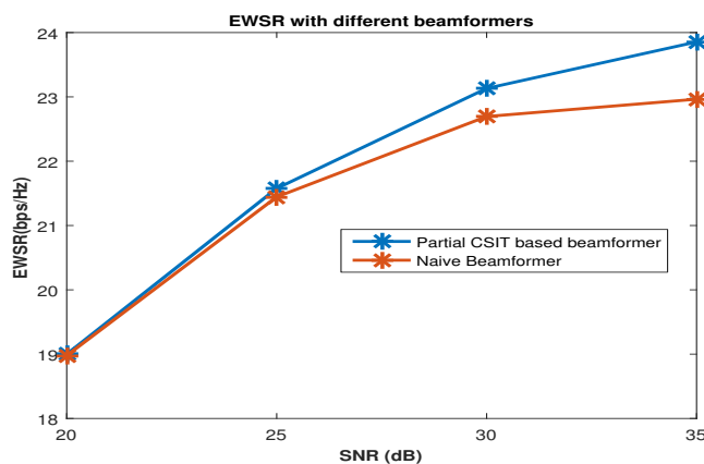
Figure 4.1: EWSR comparison for N_t = 6, N_r = 3
