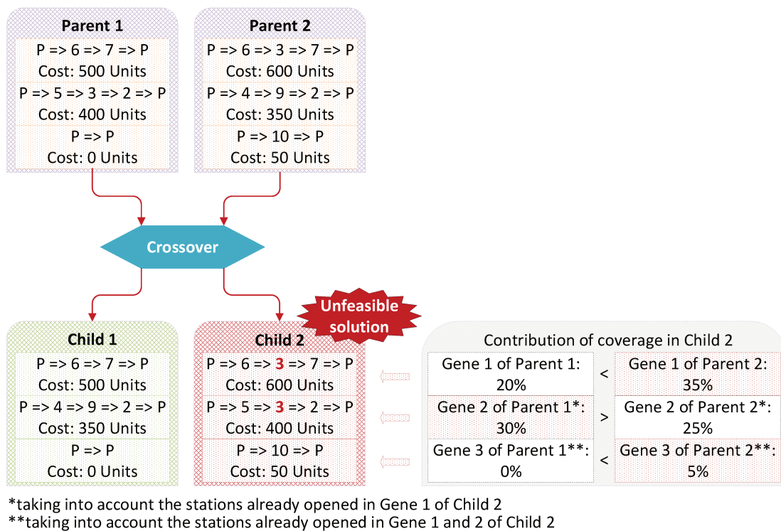
Figure 4.8: Crossover procedure
