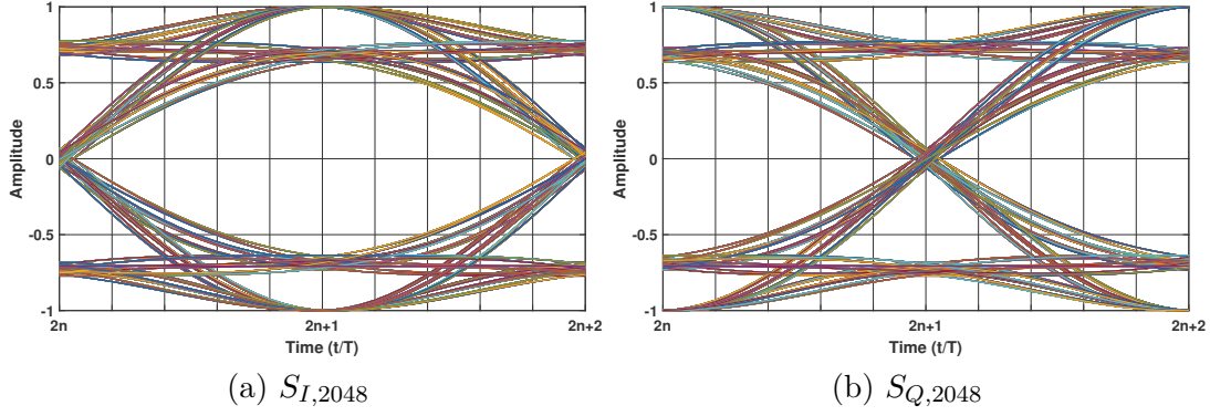
Figure 1.15 – 2048-XTCQM complex waveforms for SOQPSK-TG
