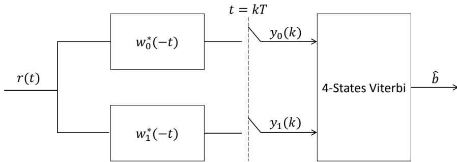
Figure 3.2 – Architecture of the Kaleh based reduced complexity detector for SOQPSK
