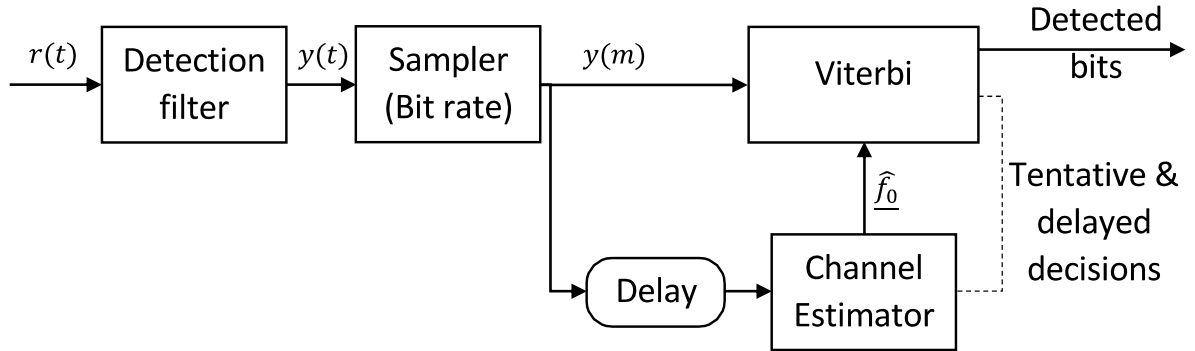
Figure 4.8 – CA-MLSD architecture
