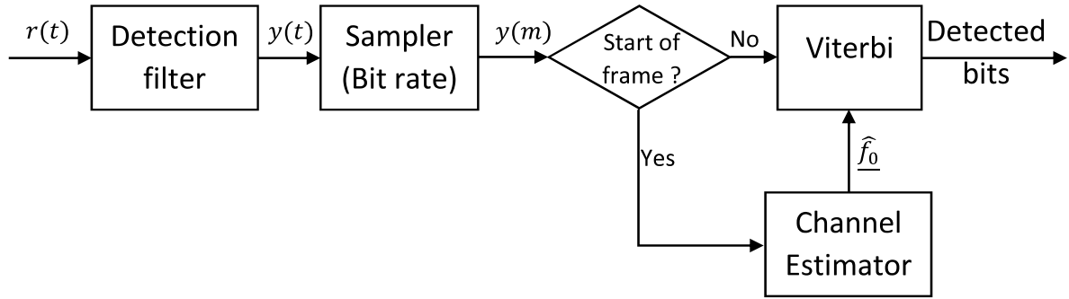
Figure 4.7 – NA-MLSD architecture
