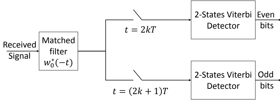
Figure 3.10 – 2x2 states detector for SOQPSK
