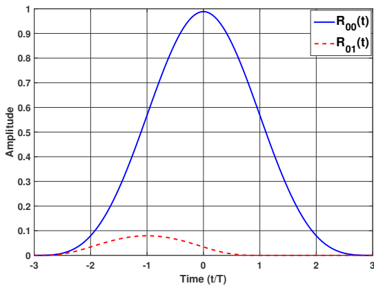
Figure 3.3 – Illustration of R_{00}(t) and R_{01}(t) for SOQPSK-MIL
