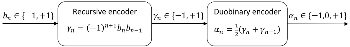
Figure 2.1 – New Vision of the SOQPSK Precoder
