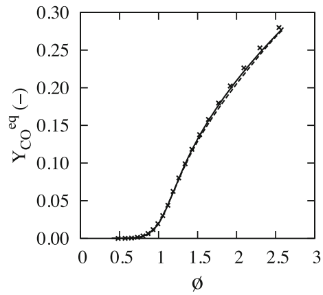
(b) CO mass fraction
