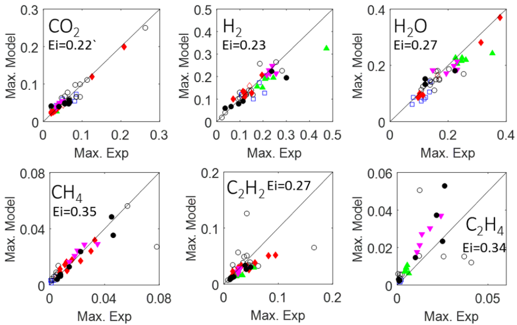
Figure 2.7: Scatter plots of the maximum calculated and measured concentration of major species. Each marker represents main fuels, \Delta : \text{CH}_4 , \square : \text{C}_2\text{H}_2 , \diamond : \text{C}_2\text{H}_4 , \nabla : \text{C}_2\text{H}_6 , and \circ : \text{C}_{3+} . Void symbol: low-pressure flames. Filled symbol: atmospheric flames. Source: Pejpichestakul et al. (2019)
