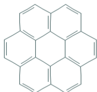
Figure 7.5: Coronene C_{24}H_{12}
