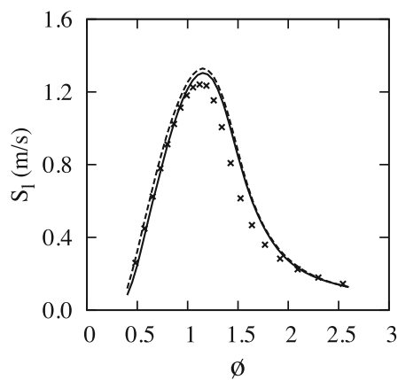
(a) Flame speed
