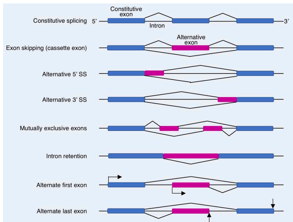
Figure 11 | Alternative splicing patterns. The different patterns of alternative splicing events that lead to inclusion or skipping of regions in mRNAs. Exons and introns that are not spliced are called constitutive. The main types of alternative splicing events are alternative 3' and 5' splice sites, cassette exons, retained introns and mutually exclusive exons. Figure adapted from (Wagner and Berglund, 2014; Wahl and Lührmann, 2015b).
