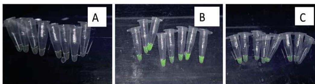
Figure 2: Screening of new Pantoea isolates using the species-specific and genus-specific LAMP tool.
