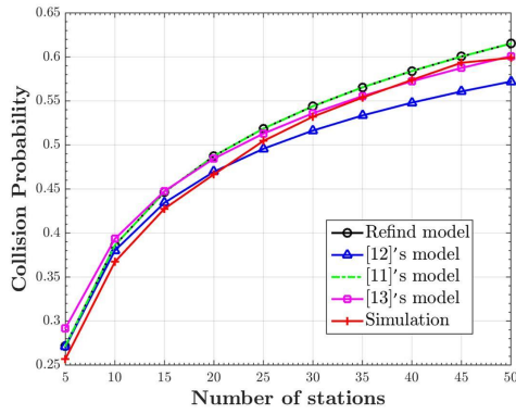
Figure 4.5: Collision probability versus network size: pksize=1500bytes and CBR=6 Mbps.
