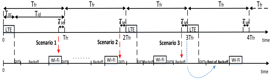
Figure 5.1: LTE interacting with Wi-Fi
