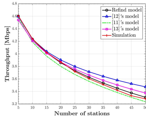
Figure 4.6: Wi-Fi throughput versus network size: pksize=1500 bytes and CBR=6Mbps.
