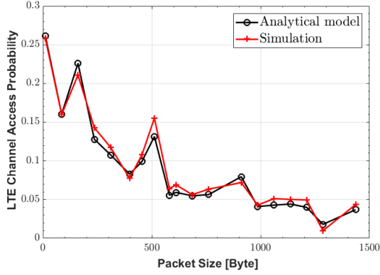
Figure 5.4: LTE channel access probability versus WiFi packet size: LTE ( T_{oc} = 1ms, T_{id} = 1ms ), WiFi (CBR = 6Mbps)
