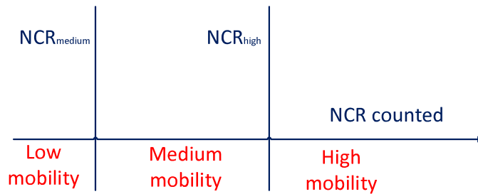
FIGURE 2.4: The 3GPP LTE MSE algorithm.
