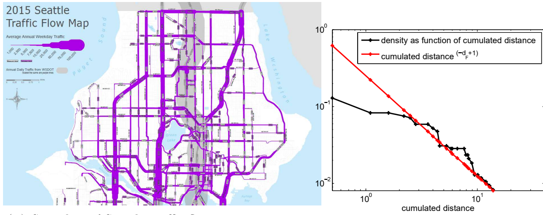
(A) Snapshot of Seattle traffic flow map (B) Computation of fractal dimension FIGURE 4.3: Procedure for Seattle
