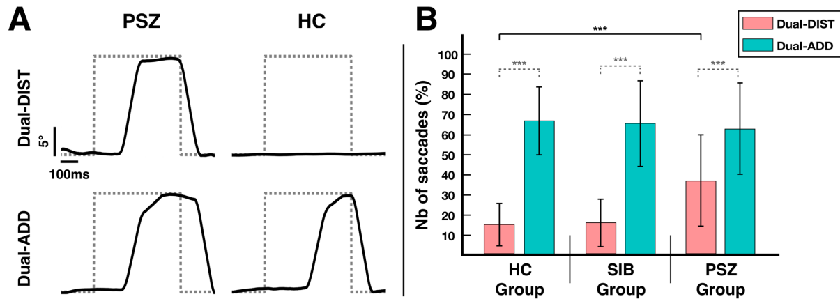
Fig 3. Saccadic execution.
