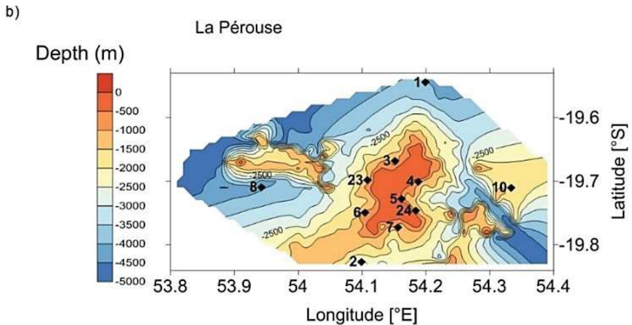
Figure 3.1(a) Map of MAD-Ridge and La Pérouse CTD stations (diamond symbols) conducted in the East African Coastal (EAFR) and Indian South Subtropical Gyre (ISSG) provinces respectively. Longhurst's (1998) biogeochemical provinces are delimited by black solid lines. Landmasses are shown in grey and seamount summits in red. (b) The La Pérouse CTD stations are plotted on the bathymetry (m). The colour bar represents the depth below the sea surface.
