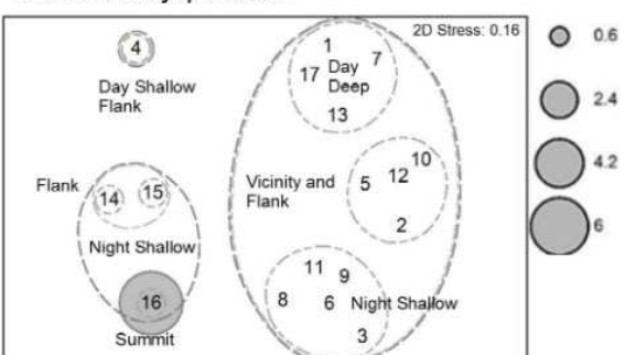
Figure 4.8 Bubble plot overlays of the MDS ordination representing the relative abundance of common (c) shallow-dwelling and vertical migratory fish species, (d) deep-dwelling, (e) and seamount summit and flank associated fish species. Trawl stations are numbered 1 to 17 on the bubble plots and dotted lines denote the 35% and 30% similarity clusters. The larger the bubble, the greater the number of individuals captured at that trawl station.
