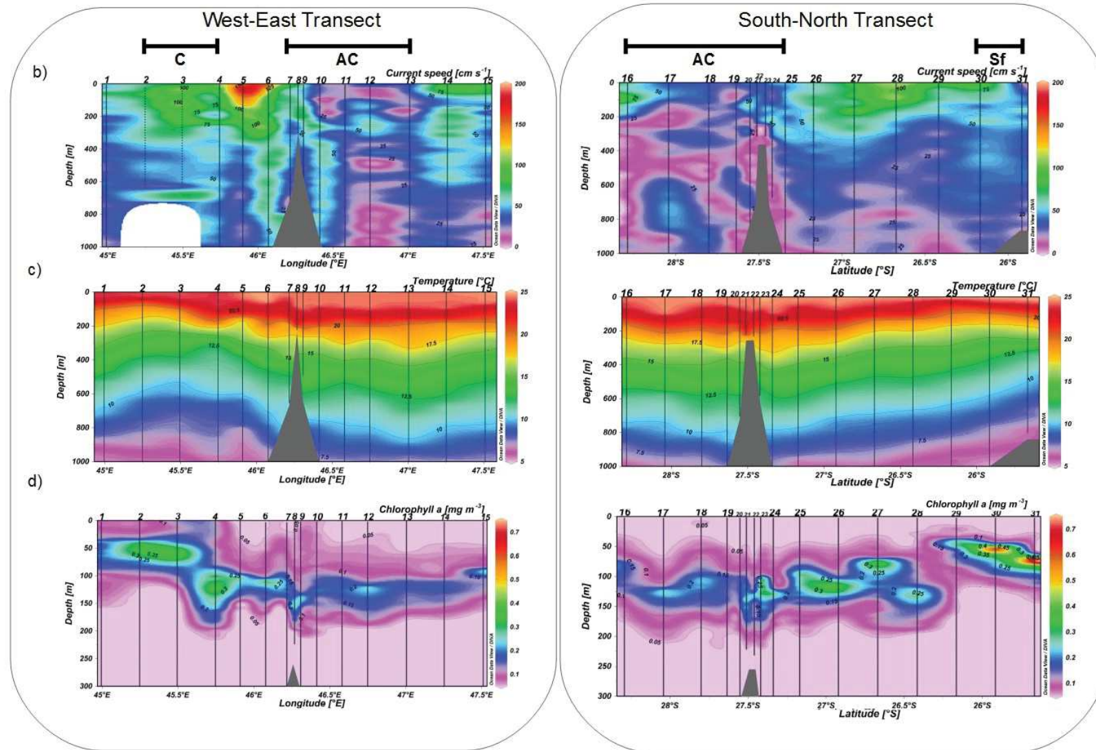
Figure 3.2 Vertical distributions of (b) current speed ( \text{cm s}^{-1} ), (c) temperature ( ^{\circ}\text{C} ), and (d) chlorophyll a ( \text{mg m}^{-3} ) for MAD-Ridge Leg 1 West-East transect (CTD stations labelled 1-15, left panels) across the cyclonic (C) and anticyclonic (AC) eddies, and South-North transect (CTD stations labelled 16-31, right panels) across the anticyclonic eddy and on the Shelf (Sf). The MAD-Ridge seamount and the Madagascar shelf are shown in grey.
