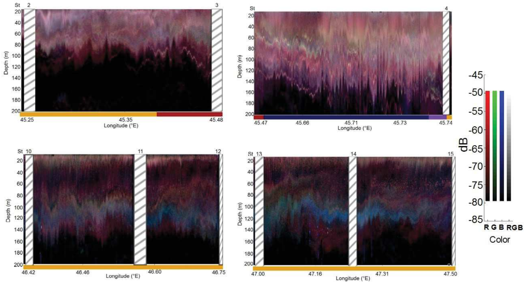
Figure 3.3(c) RGB composite images of Sv values (dB re 1 m -1 ) across cyclonic CTD stations 2-3 and 4 and anticyclonic stations 10-12 and stations 13-15 (denoted by striped bars). The 38, 70 and 120 kHz frequencies were given red, green and blue colour codes, respectively, as explained in the methods. Periods corresponding to sunset, night, sunrise and day are denoted by red, blue, violet and gold horizontal rectangles, respectively.
