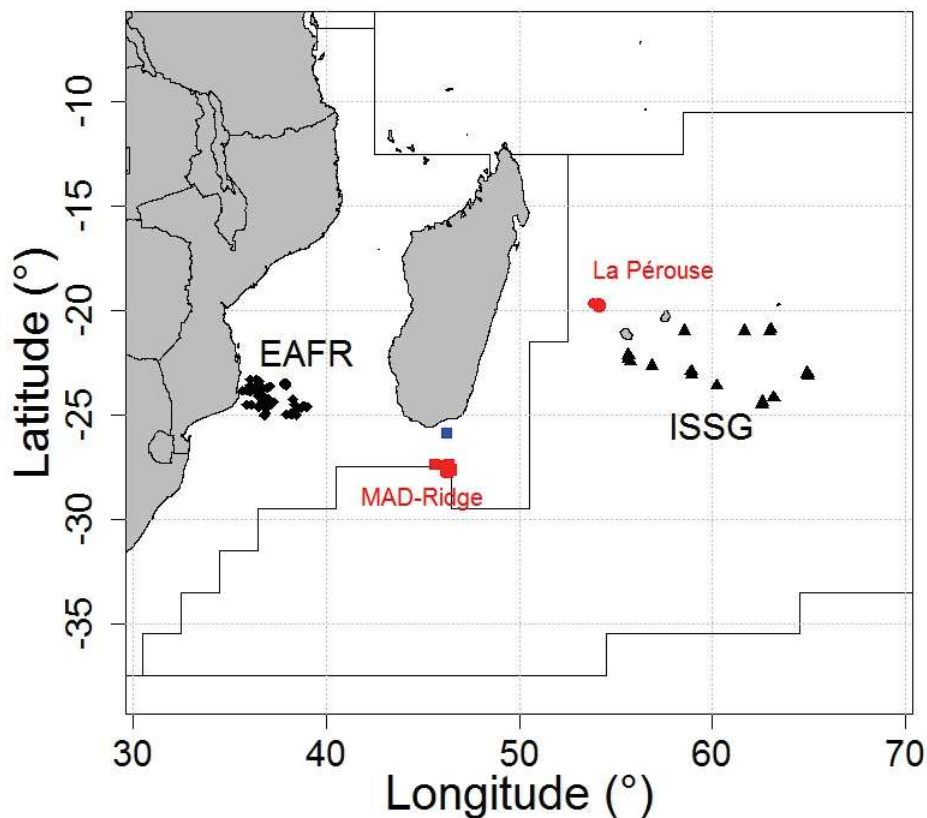
Figure 6.1(a) Map of the MICROTAN stations (black triangles) and La Pérouse seamount (red dot) in the ISSG province, of the MESOP 2009 stations (diamond symbols) (Annasawmy et al., 2018), Madagascar shelf station (blue square) and MAD-Ridge stations (red squares) in the EAFR province. Longhurst's (2007) biogeochemical provinces (ISSG and EAFR) are delimited by black solid lines.
