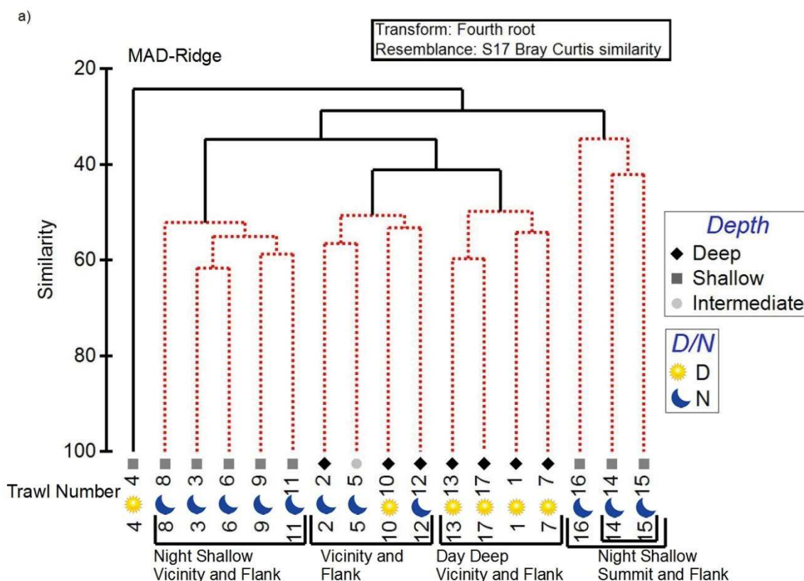
Figure 4.8(a) Similarity cluster dendrogram of species abundance at MAD-Ridge trawl stations 1 to 17. Brackets represent cluster groups at 35% (Night shallow, vicinity and flank; Day deep, vicinity and flank); and 30% similarities (Night shallow, summit and flank).
