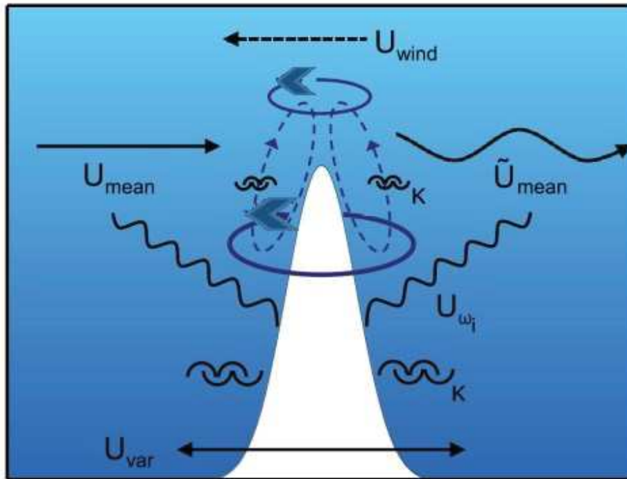
Figure 1.2 Characteristic features of motion at an isolated southern hemisphere seamount. These features, including a vertical circulation cell, isopycnal doming and anticyclonic-horizonal circulation, are shown near the summit depth, superimposed on oscillatory currents and oscillatory temperature and salinity distributions. The occurrence, properties and variability of these features depend on local turbulence K , internal waves U_{\omega_i} (propagating horizontally and vertically), and on incident mean current U_{mean} , eddies \tilde{U}_{mean} , tidal and other oscillations U_{var} , and possibly wind-driven currents U_{wind} (Source: adapted from Lavelle & Mohn, 2010).
