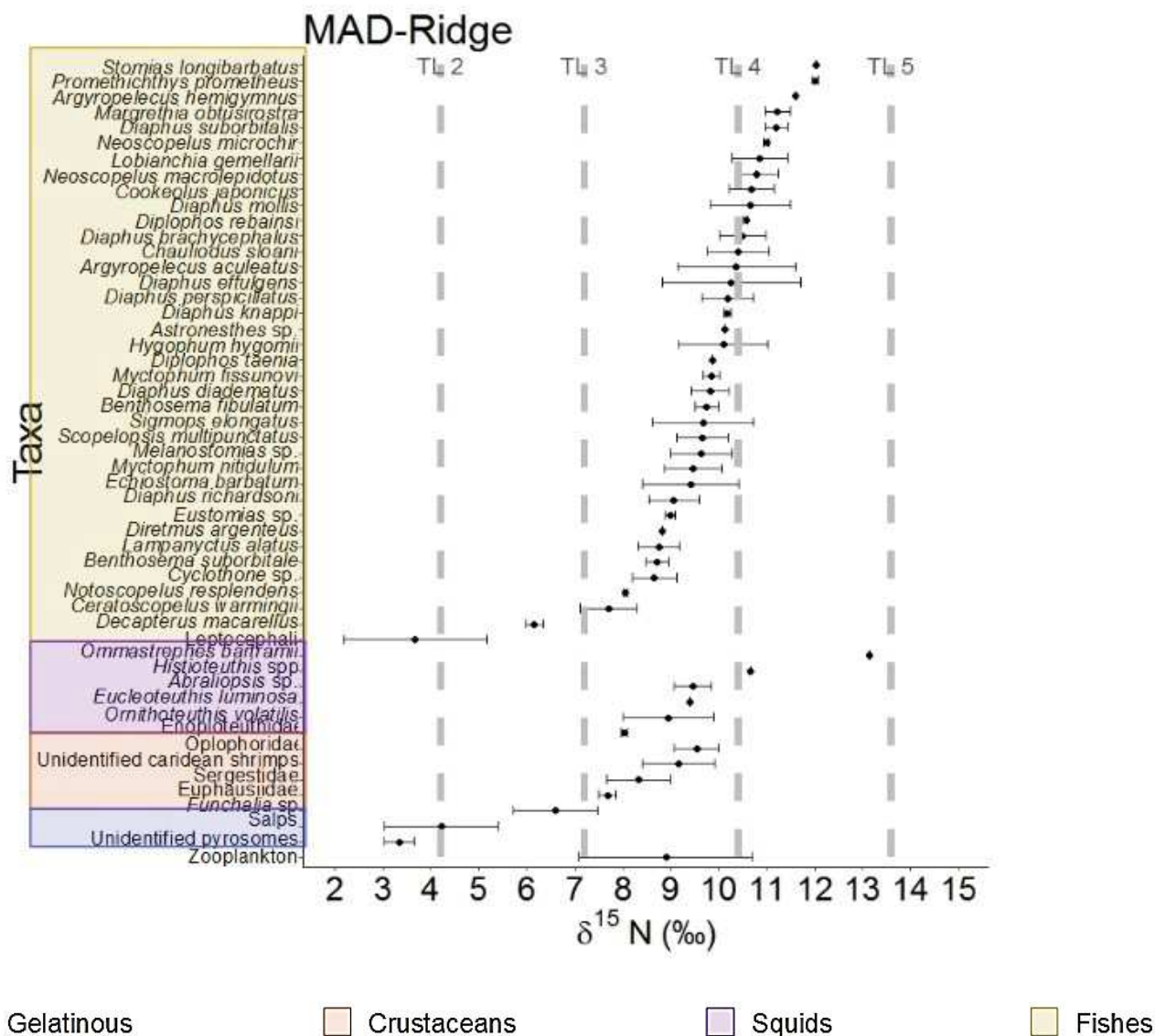
Figure 5.5(b) \delta^{15}\text{N} (mean \pm S.D.) values (‰) and estimated trophic level (TL as estimated from the TPA method) of POM-Surf, POM-Fmax, zooplankton, gelatinous and sampled micronekton species at the MAD-Ridge seamount. Taxa are placed in their broad categories and \delta^{15}\text{N} compositions are sorted in ascending order of their values.
