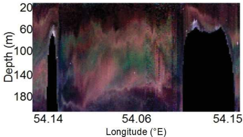
Figure 3.7 RGB composite images of S_V values ( \text{dB re } 1 \text{ m}^{-1} ) of (c) La Pérouse day, (d) MAD-Ridge day, (e) La Pérouse night and (f) MAD-Ridge night. The MAD-Ridge and La Pérouse summits are shown in black. The 38, 70 and 120 kHz frequencies were given red, green and blue colour codes respectively. Regions of high S_V are denoted by “white patches” on the RGB composites.
