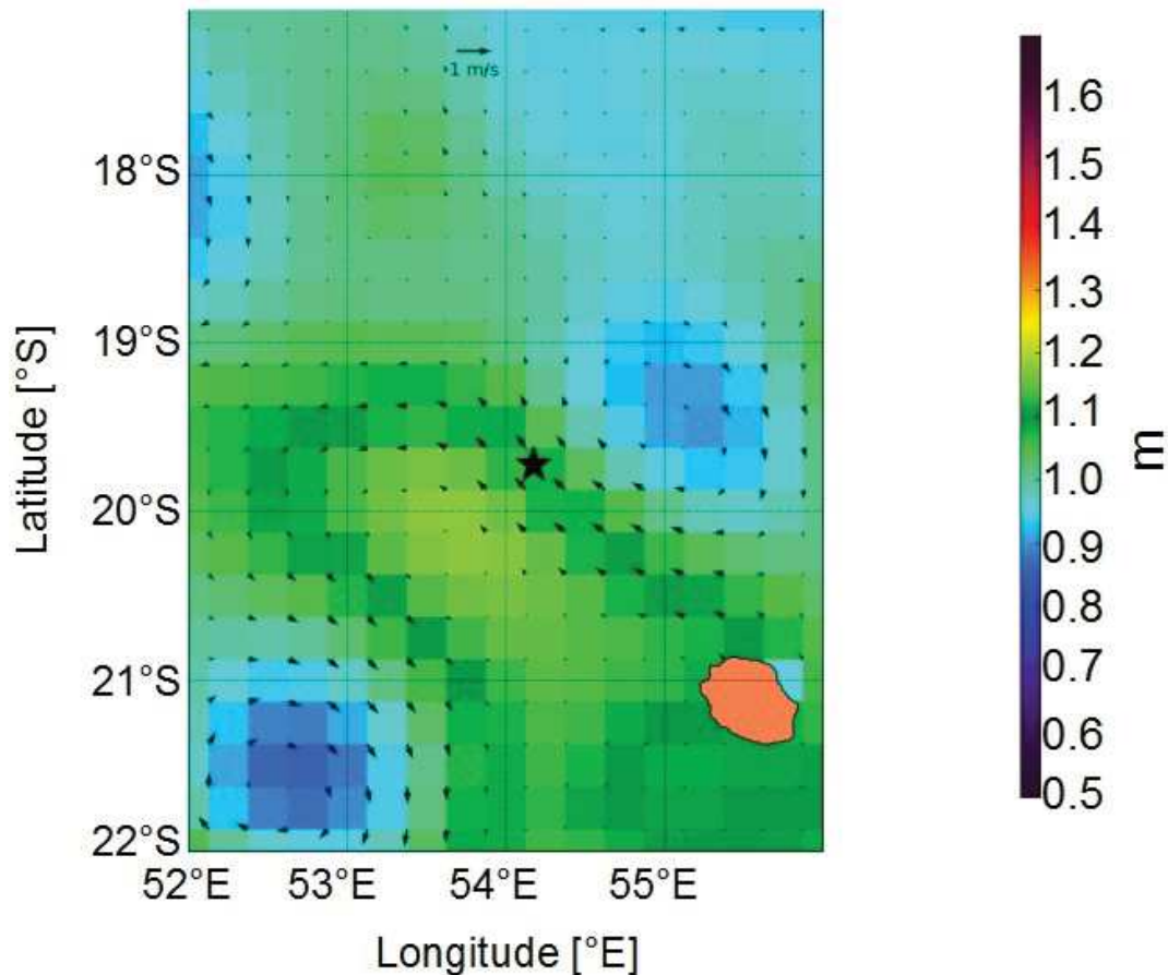
Figure 3.6 Satellite surface absolute dynamic height (m) on 16 September 2016 during the La Pérouse cruise showing La Pérouse seamount (black star). Geostrophic velocity vectors ( m s^{-1} ) (black arrows) are superimposed. Réunion landmass is shown in orange.
