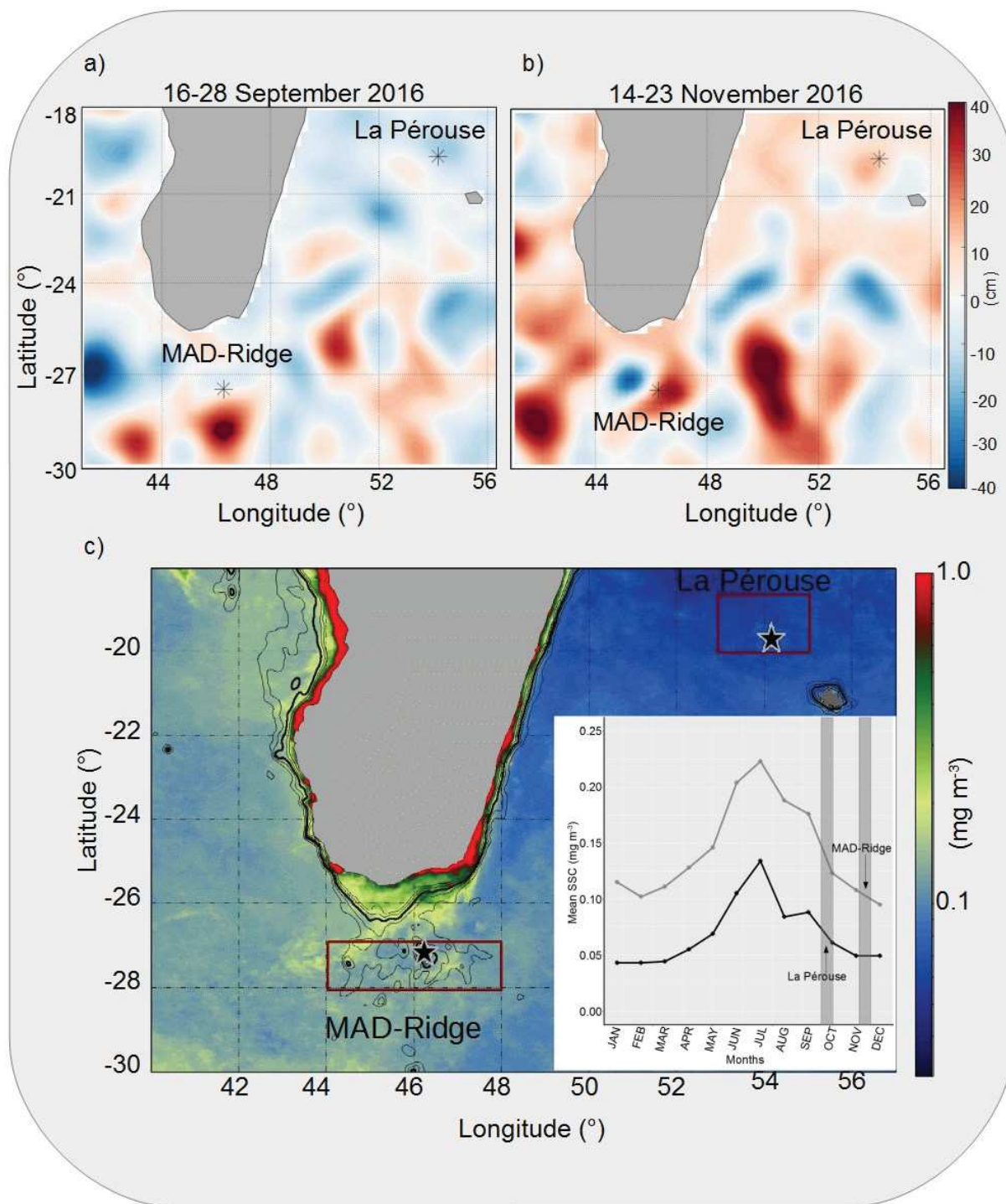
Figure 4.2 Averaged sea level anomaly (MSLA) map, with La Pérouse and MAD-Ridge seamounts shown as black star symbols, and dated (a) 16-28 September 2016, (b) 14-23 November 2016. The colour bar indicates the SLA in cm, with positive SLA (red) and negative SLA (blue). (c) Averaged satellite image of surface chlorophyll a distribution from 18/09/2016 to 07/12/2016. Monthly mean surface chlorophyll a values for the region defined by the red squares are depicted from January to December 2016. The dates of La Pérouse and MAD-Ridge cruises are marked by grey bars on the monthly mean plot. The colour bar indicates the surface chlorophyll a concentration in \text{mg m}^{-3} .
