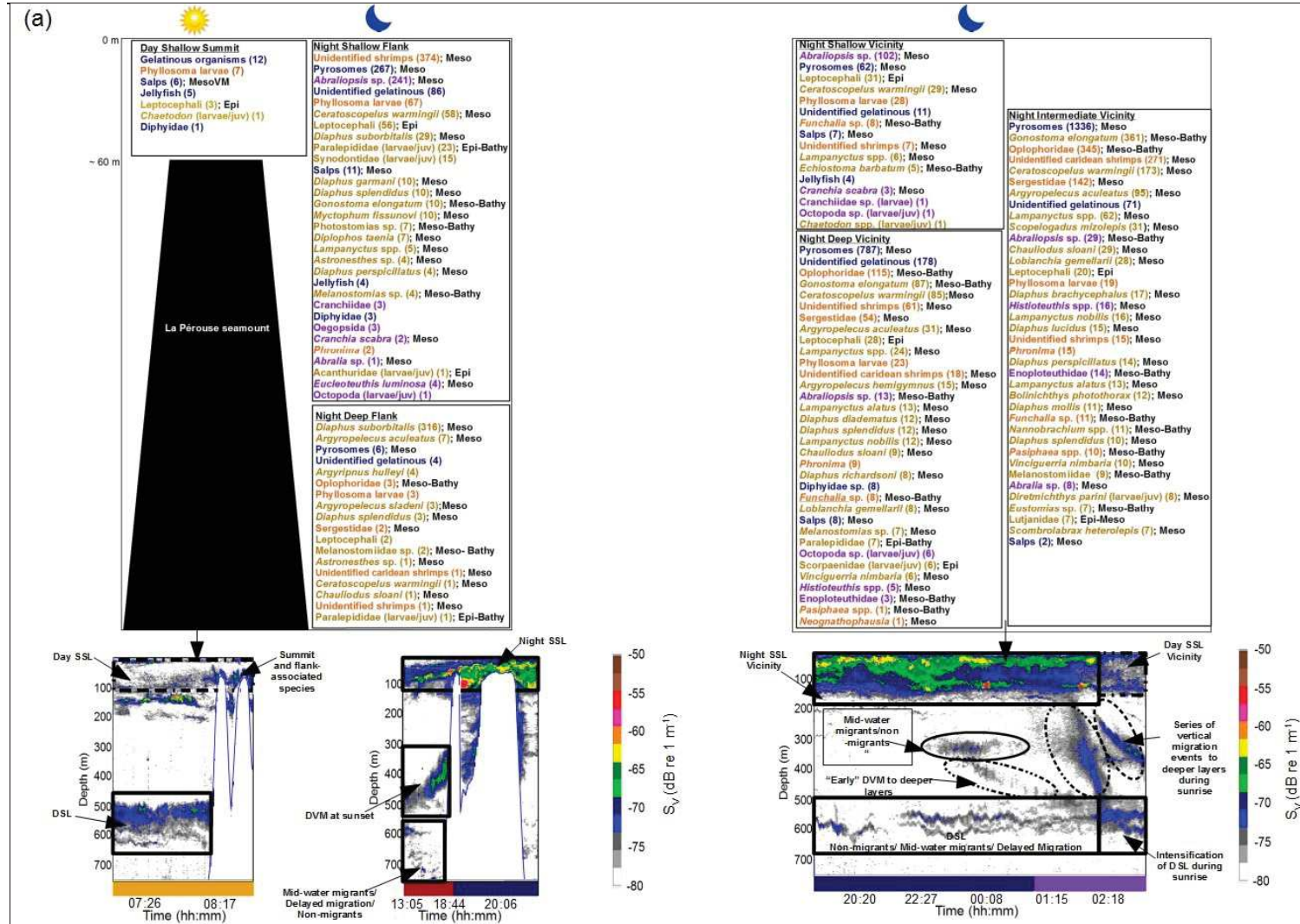
Figure 4.9(a) Schematics of La Pérouse seamount, listing the most dominant taxa (gelatinous organisms in blue, crustaceans in orange, cephalopods in violet and fishes in yellow), within the cluster groups. The numbers in brackets indicate the number of individuals caught. Organisms are classified as being epi (epipelagic), meso (mesopelagic), bathy (bathypelagic) and benthic (benthopelagic). Echograms of the 38 kHz frequency at sunset, night, sunrise and daytime are denoted by red, blue, violet and gold coloured rectangles respectively. The series of DVM events from the intermediate layer and from the SSL are denoted by circular dotted lines. The night SSL and day SSL are denoted by solid and dotted rectangles respectively. The DSL is denoted by solid rectangles. Backscatter from seamount-associated species are also noted. The colour bar indicates Sv in dB re 1 m -1 .
