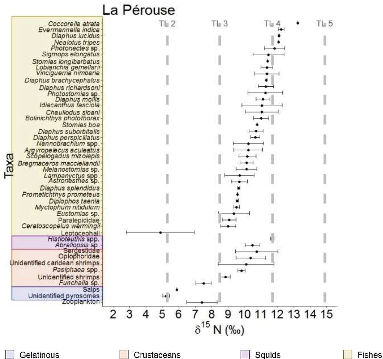
Figure 5.5(a) \delta^{15}N (mean \pm S.D.) values (‰) and estimated trophic level (TL as estimated from the TPA method) of POM-Surf, POM-Fmax, zooplankton, gelatinous and sampled micronekton species at the La Pérouse seamount. Taxa are placed in their broad categories and \delta^{15}N compositions are sorted in ascending order of their values.
