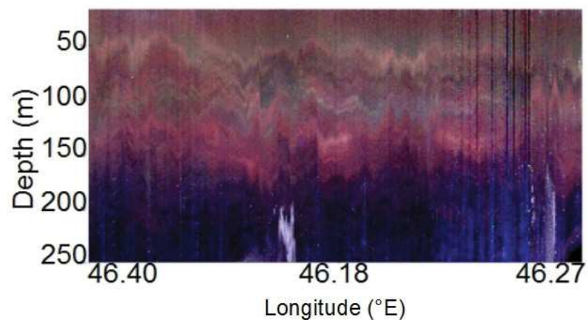
Figure 3.7 RGB composite images of S_V values ( \text{dB re } 1 \text{ m}^{-1} ) of (c) La Pérouse day, (d) MAD-Ridge day, (e) La Pérouse night and (f) MAD-Ridge night. The MAD-Ridge and La Pérouse summits are shown in black. The 38, 70 and 120 kHz frequencies were given red, green and blue colour codes respectively. Regions of high S_V are denoted by “white patches” on the RGB composites.
