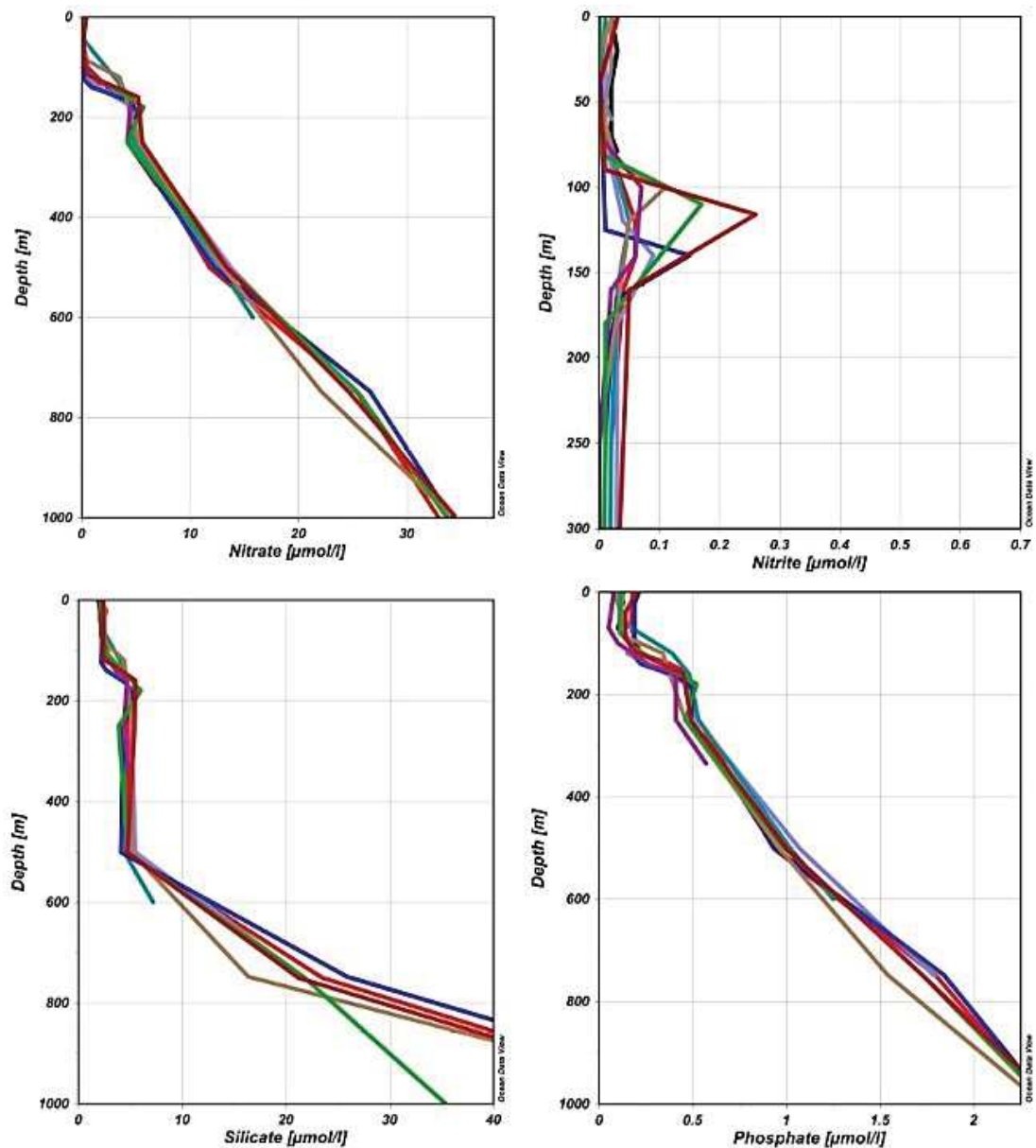
Figure 2.18 Vertical profiles of nitrate, nitrite, silicate and phosphate in \mu\text{mol l}^{-1} at La P erouse seamount.
