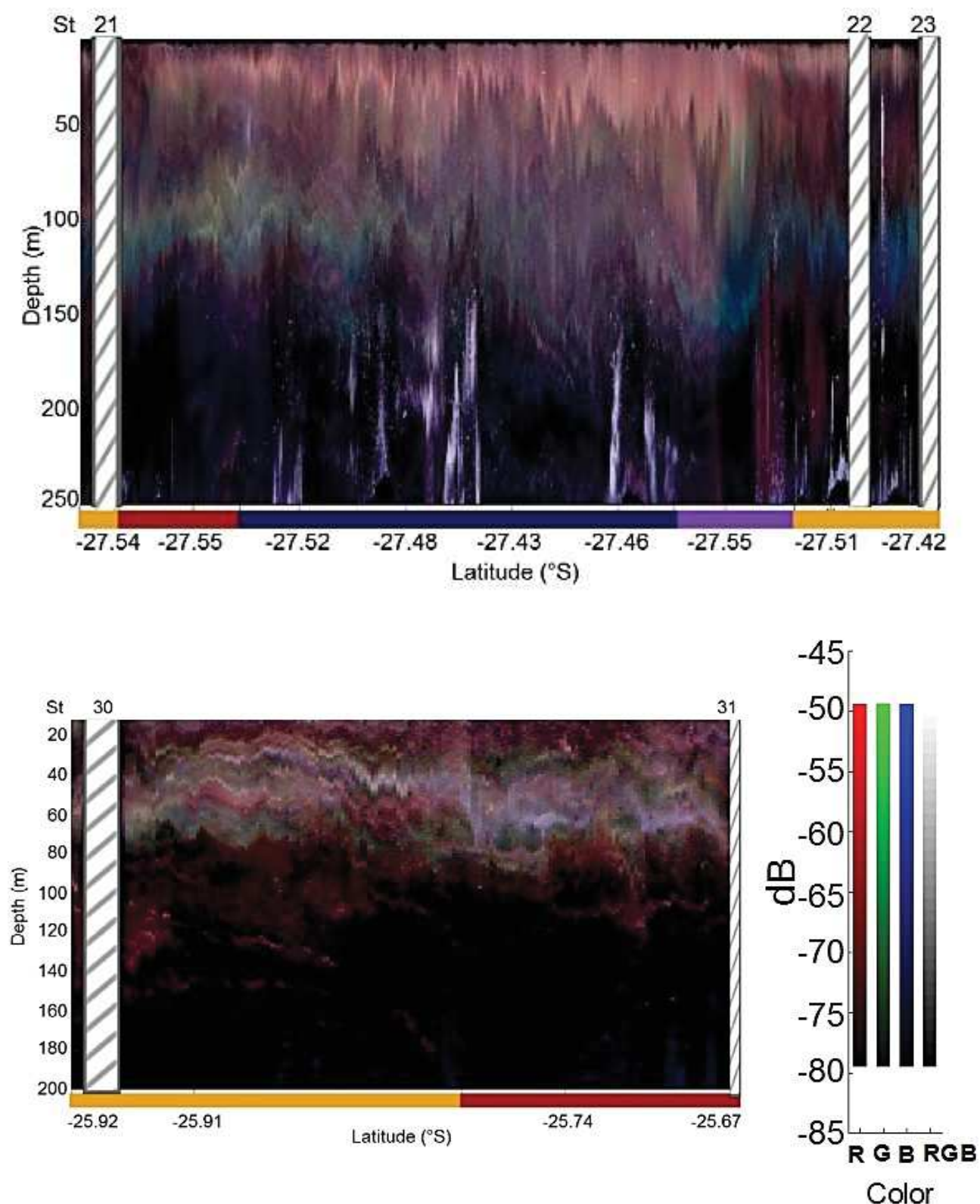
Figure 3.4(b) RGB composite images of Sv values ( \text{dB re } 1 \text{ m}^{-1} ) at anticyclonic CTD stations 21-23 and shelf stations 30-31 (labelled by striped bars). The 38 kHz, 70 kHz and 120 kHz frequencies were given red, green and blue colour codes, respectively. Periods corresponding to sunset, night, sunrise and day are denoted by red, blue, violet and gold horizontal rectangles, respectively on the plots.
