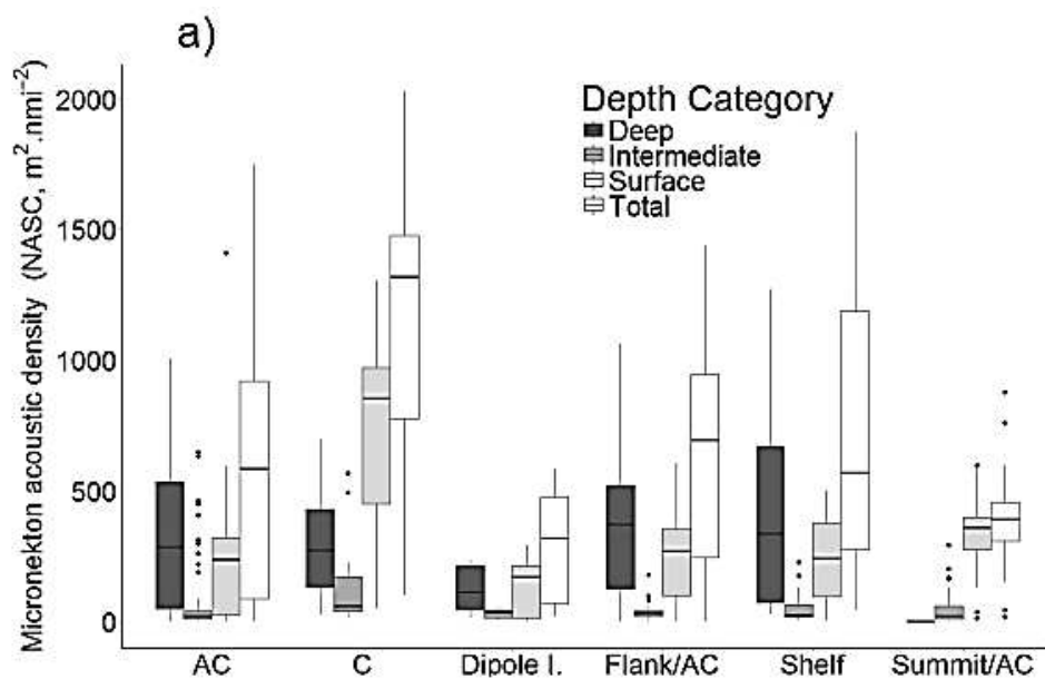
Figure 3.5(a) Boxplots of the total micronekton acoustic densities ( s_A, \text{m}^2 \text{ nmi}^{-2} ) of the 38 kHz frequency in the deep (400–735 m), intermediate (200–400 m), surface layers (10–200 m) and total water column (10–735 m) for the transects at CTD stations: 10–13, 16–19, 24, 25 (AC: anticyclonic); 2, 3, 4 (C: cyclonic); 5 (Dipole Interface); 7, 9, 20, 23 (Flank/AC); 30, 31 (Shelf); and 8, 21, 22 (Summit/AC) of the MAD-Ridge cruise.
