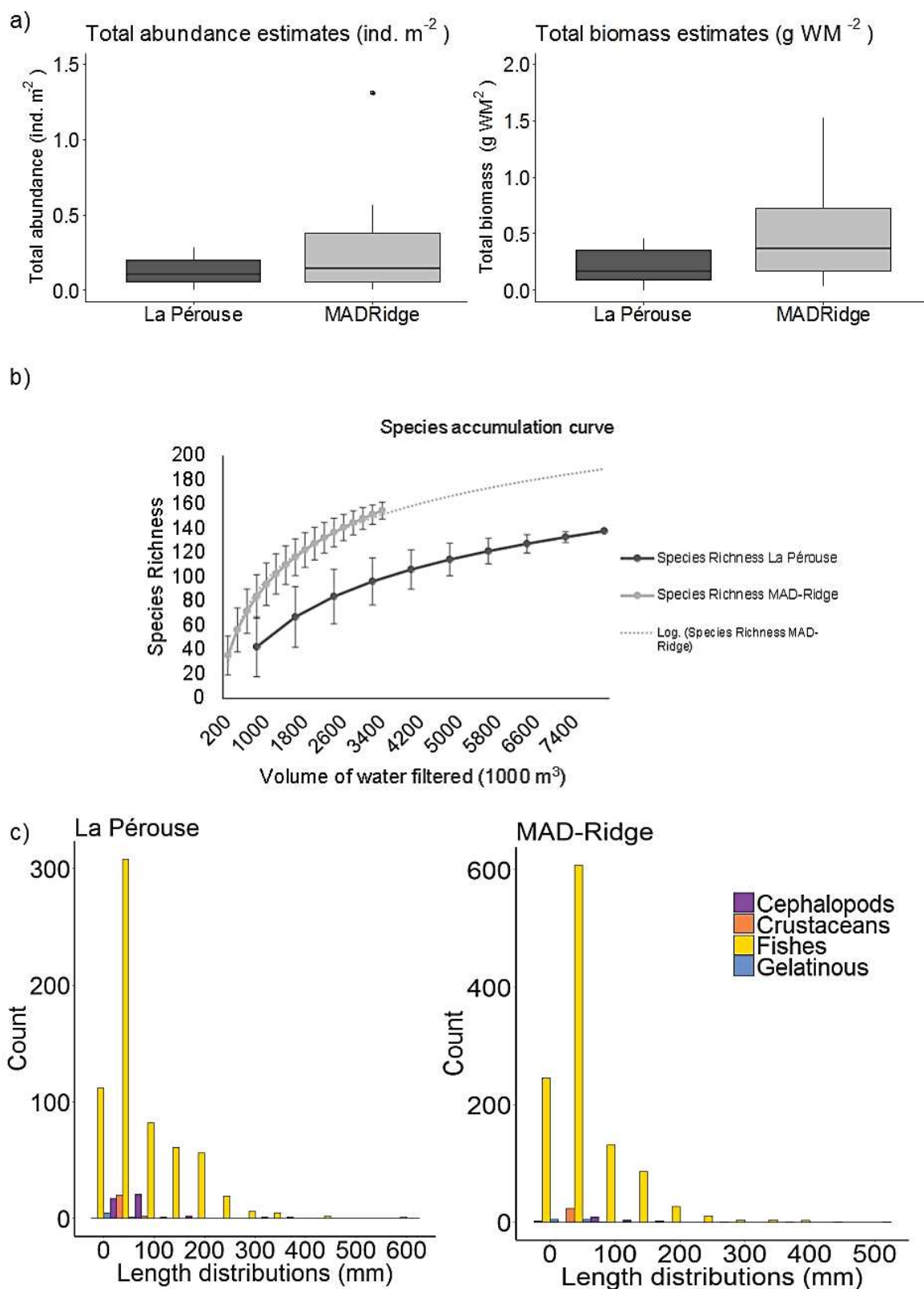
Figure 4.6 At La Pérouse and MAD-Ridge seamounts, (a) boxplot of total abundance and biomass estimates (in ind m^{-2} and g WM^{-2} respectively), (b) species richness with increasing sampling effort (volume of water filtered in 1000 m^3 ), (c) length distributions of selected gelatinous plankton, crustaceans, cephalopods and epi-mesopelagic fishes sampled.
