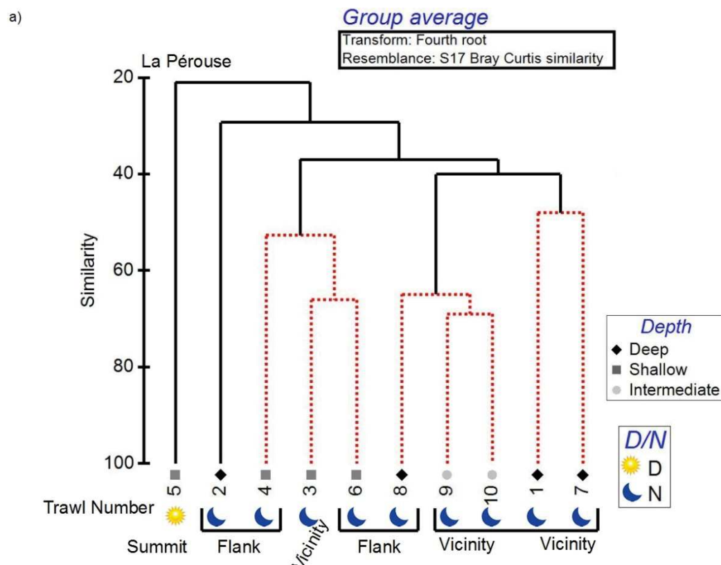
Figure 4.7(a) Similarity cluster dendrogram of species abundance at La Pérouse trawl stations 1 to 10. Brackets represent cluster groups at 42% (Day shallow summit, Night deep flank, night shallow vicinity and flank; night intermediate vicinity and Night deep vicinity).
