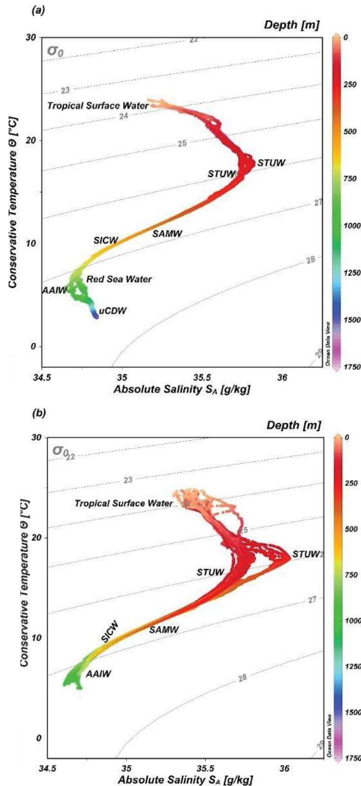
Figure 2.2 Temperature-Salinity diagrams indicating the water masses in the SWIO. Conservative Temperature ( ^{\circ}\text{C} ) vs. Absolute Salinity ( \text{g kg}^{-1} ) (as in Vianello et al., 2020) profiles (a) to the North West of Réunion Island, and (b) south of Madagascar, showing the AAIW (Antarctic Intermediate Water), SICW (South Indian Central Water), SAMW (Sub-Antarctic Mode Water), STUW (Subtropical Under Water) and Tropical surface Waters. The Red Sea Water and uCDW (upper Circumpolar Deep Water) were observed to the north-west of Réunion Island.
