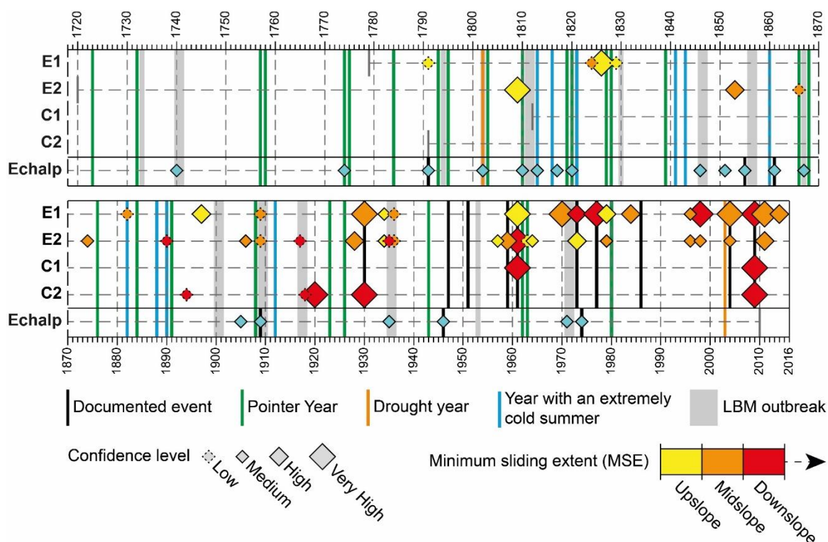
Figure 3.7 – Avalanche events reconstructed for the period 1720-2016 at the four avalanche paths. Symbol sizes are proportional to the level of confidence, whereas the color range denotes the minimum slide extent. Grey bands represent years associated to LBM outbreaks. Vertical lines show snow avalanche events documented in historical archives (black), as well as extremely dry (orange), cold (blue) summers and pointer years (green).
