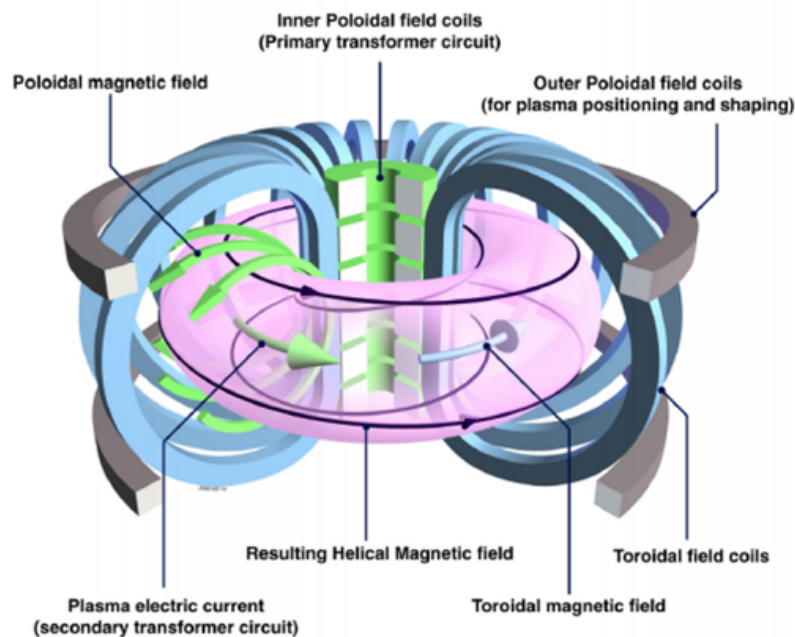
Figure 1.4: Simplified tokamak structure -
