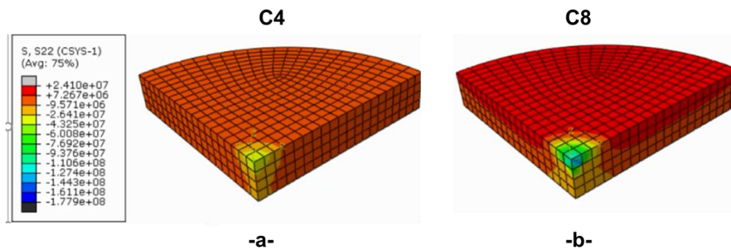
Figure B-6: Secondary principal stress obtained from numerical simulation in a) C4 and b) C8
