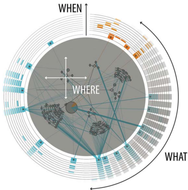
Figure 3.5: VisAlert [74]
