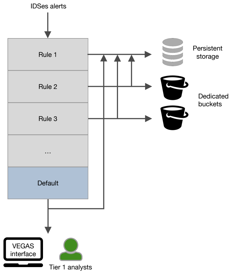
Figure 4.2: VEGAS workflow.
