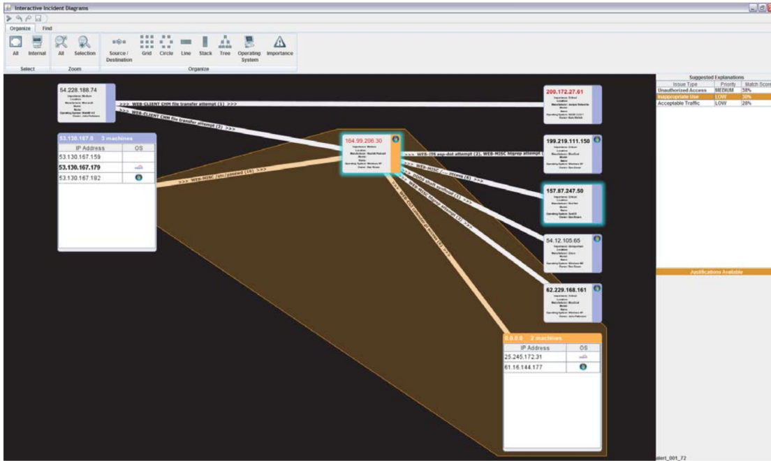
Figure 3.4: NIMBLE interface [71]
