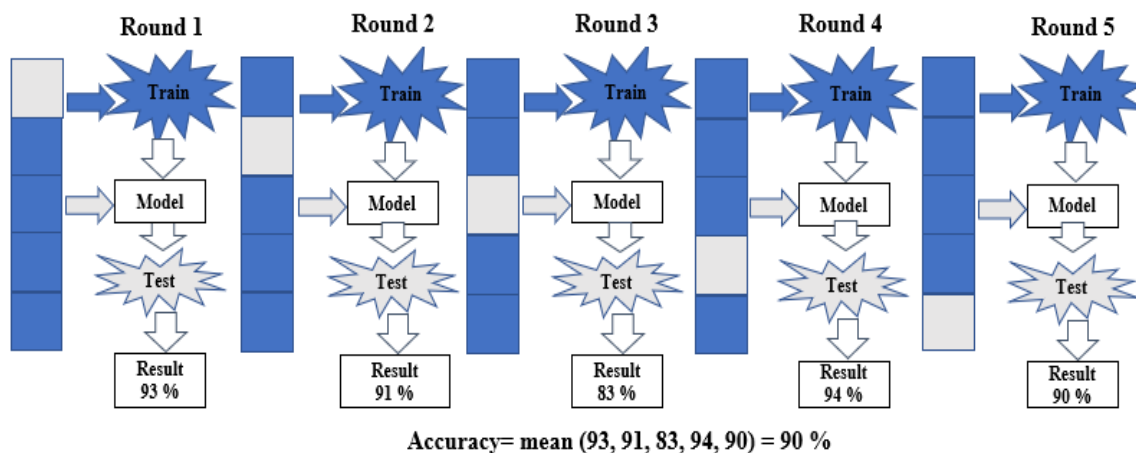
Figure 2-15 5-Fold Cross-Validation [106].
