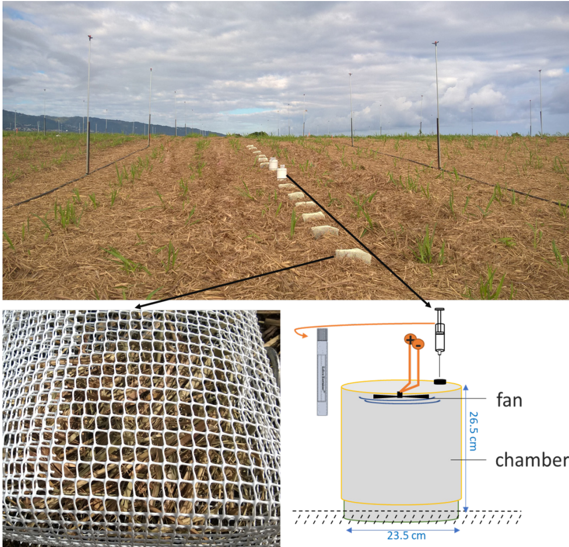
Figure 1: Design of litterbag and gas chamber experiments, measuring the decomposition and the emissions of \text{CO}_2 and \text{N}_2\text{O} of mulch-fertilizers mixtures on field. View of a plot with two quantities of sugarcane mulch.
