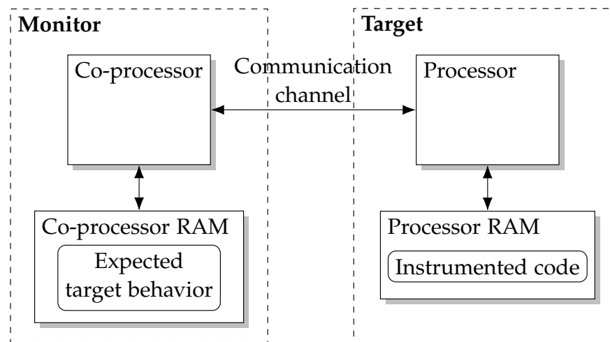
Figure 9.1: High-level overview of our co-processor-based monitoring approach
