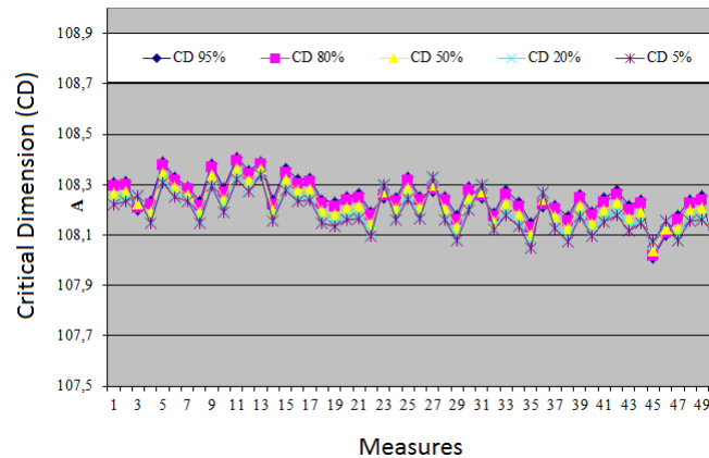
Figure 3.4 – Repeatability chart for a CD measure, 50 measures were performed at the same point (STMicronics).
