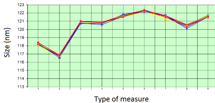
Figure 3.5 – Reproducibility chart for 9 different measures. One measurement done per day on the same wafer (STMicronics).
