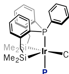
3-7 PPh_3 3-3a PCy_3
