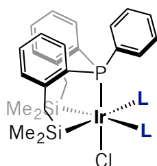
3-2a CO 3-3a piridina- d_5 3-4a CD_3CN 3-5a PhCN
