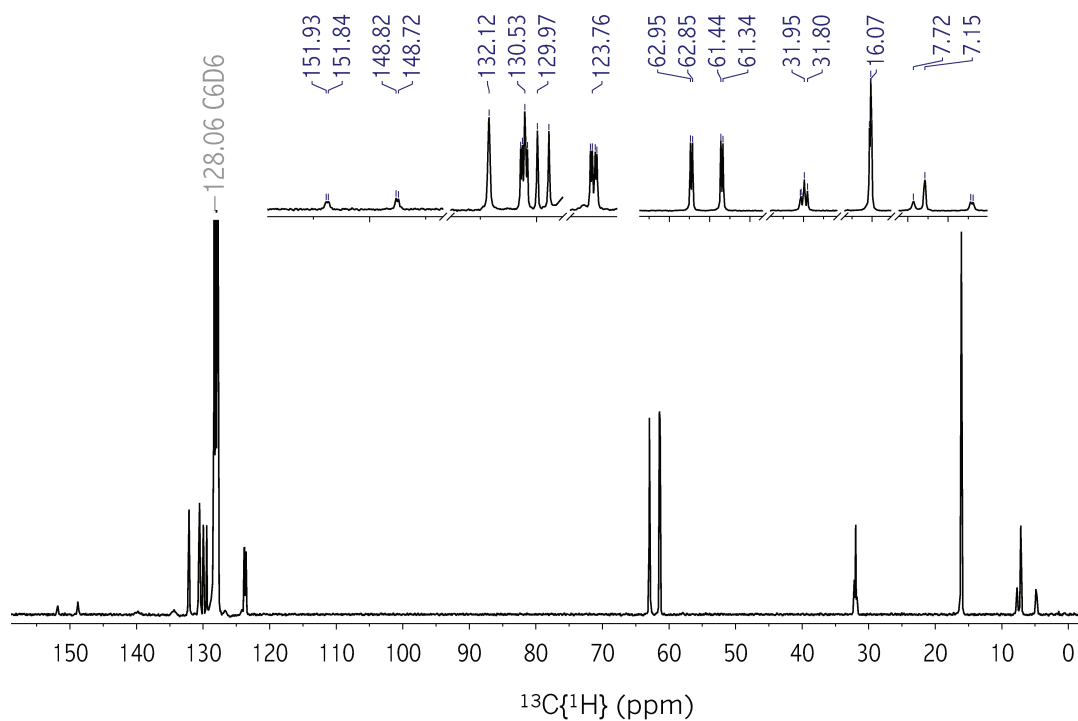
Figura 3A.19 RMN de ^{13}\text{C}\{^1\text{H}\} (100.6 MHz, 298 K, \text{C}_6\text{D}_6 ) correspondiente al complejo 3-6b .
