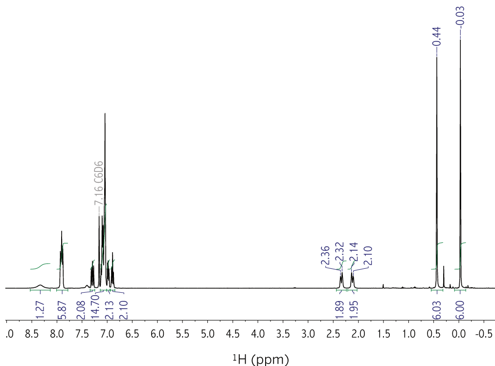
Figura 3.33 Espectro de RMN de ^1\text{H} (400 MHz, 298 K, \text{C}_6\text{D}_6 ) correspondiente al complejo [(\text{SiPSi})\text{Ir}(\text{Cl})(\text{PPh}_3)] 3–7 .
