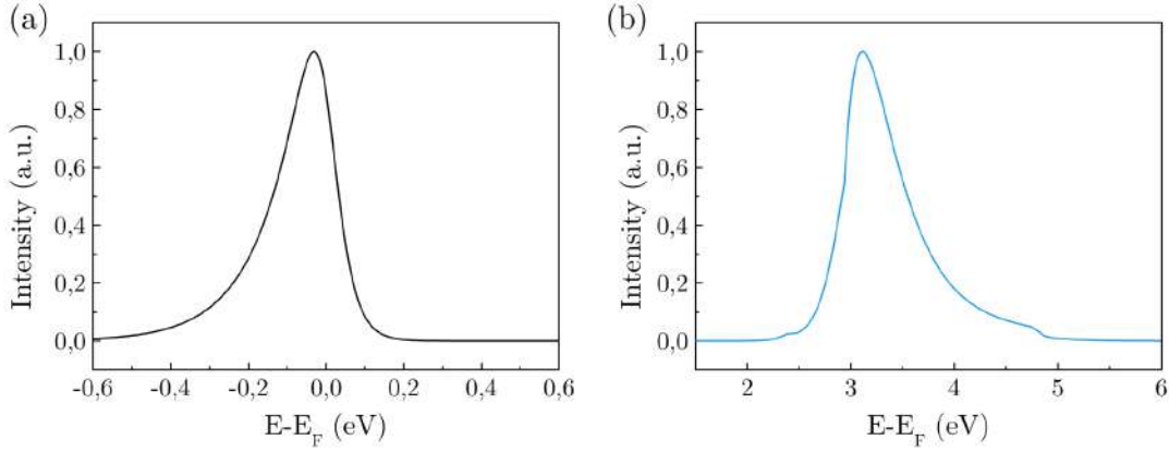
Figure 1.19: (a) Simulated ZLP of a CFEG TEM working in DC mode. (b) Simulated ZLP of our CFEG based TEM operated in pulsed mode ( E_{ph} = 2.4 \text{ eV} , F_{loc} = 1.19 \text{ V/nm} ). The spectrum has been obtained by integrating the electron energy distribution over the laser pulse duration.
