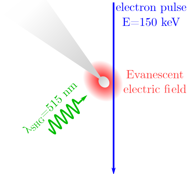
Figure 3.2: Schematic representation of the electron-photon interaction obtained in FemtoTEM. The nanosized extremity of the tungsten emitter has been used to create the evanescent electric field.
