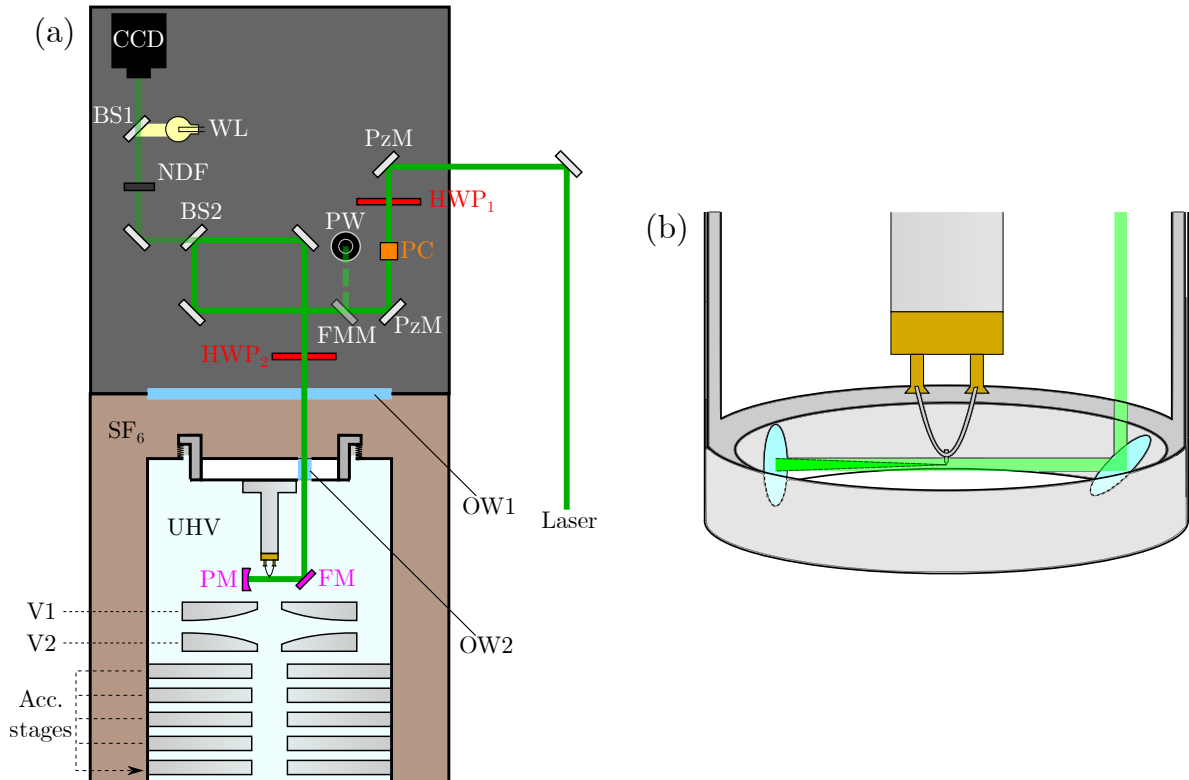
Figure 2.2: (a) Ultrafast CFEG and optical head. HWP: Half-Wave Plate. FMM: Flip Mount Mirror. PW: Power meter. PzM: Piezoelectric Mirror. BS: Beam Splitter. WL: White Light source. OW: Optical Window. FM: Flat Mirror. PM: Parabolic Mirror. PC: Polarizing Cube. (b) Sketch of the CFEG tip mounted on a HHT support and the mirror holder.
