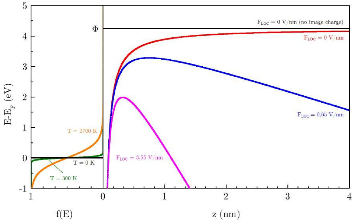
Figure 1.10: Left side. Fermi-Dirac (F-D) distribution at three different temperatures: T = 0 K (black curve), T = 300 K (green curve), T = 2700 K (orange curve) that is the typical temperature used for thermionic emission from tungsten. Right side. Potential barrier at a metal-vacuum interface for \langle 310 \rangle -oriented tungsten ( \phi = 4.25 eV) for different values of the applied electric field. The black curve represents the potential barrier without any applied electric field and neglecting the image charge contribution. The coloured curves take into account the image charge in three cases: no applied field (red), Schottky electron gun F_{LOC} = 0.65 V/nm (blue) and Cold Field Emission Guns F_{LOC} = 3.55 V/nm (magenta). z is perpendicular to the metal surface.
