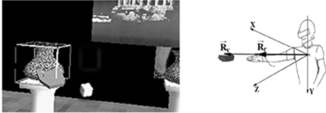
FIGURE 18 – Left : The Go-Go Technique, Right : The vector R_r represents the real hand position and the vector R_v represents the virtual hand position
