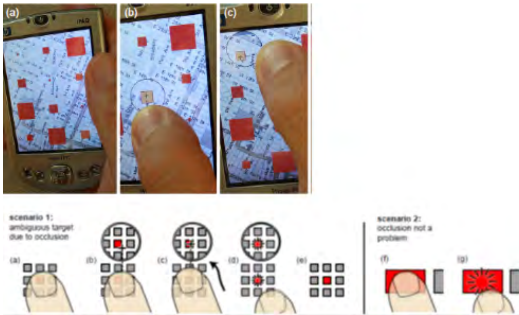
FIGURE 41 – Shift interaction technique and design
