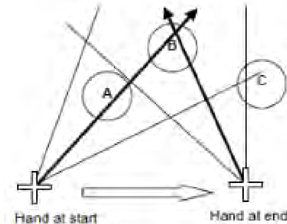
FIGURE 27 – The shadow cone interaction technique. A and B are highlighted at the start than A is dropped after the modification of the hand position
