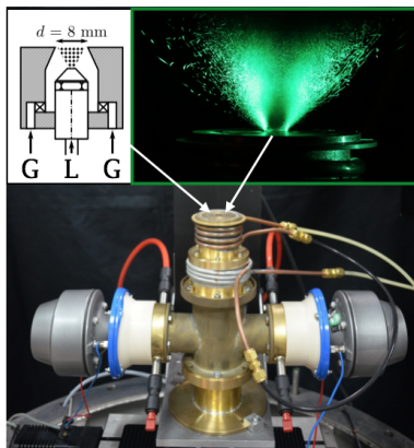
Figure 1: Experimental burner. A sketch of the swirl injector appears in the top left-hand corner and a vertical tomography of the spray is shown in the top right-hand corner.
