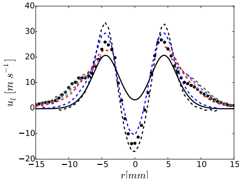
Figure 6: Mean axial velocity field for the liquid phase at x = 7.5 mm. —: Numerical results; ●: Mass-averaged experimental field; Experimental profiles: - - : d_l = 2 - 3 \mu\text{m} ; - · - : d_l = 10 - 12 \mu\text{m} ; - · - : d_l = 20 - 23 \mu\text{m} ; - · - : d_l = 23 - 36 \mu\text{m} ; - · - : d_l = 26 - 30 \mu\text{m} ; - · - : d_l = 30 - 34 \mu\text{m} ;
