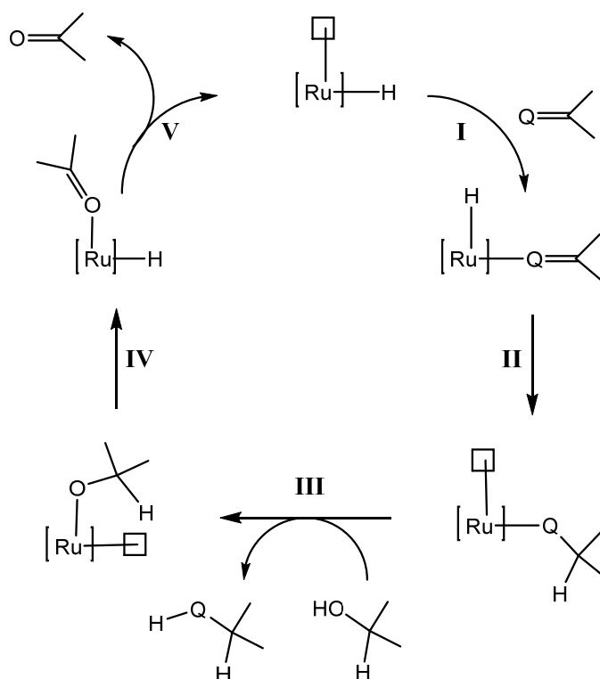
Scheme 13. The inner sphere mechanism of TH (Q = O, NH).
