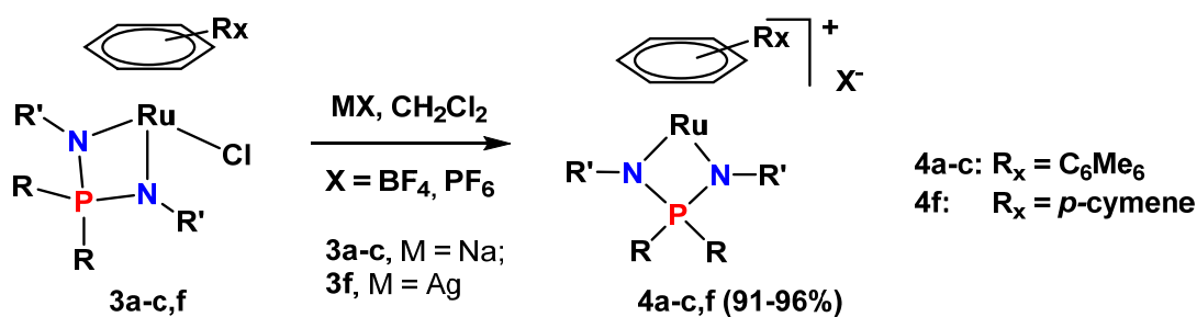
Scheme 25. Synthesis of 16e ruthenium cationic NPN complexes 4a-c,f .
