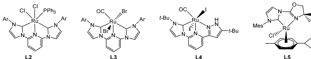
Figure 1. Ruthenium catalysts containing NHC-ligands for TH.
