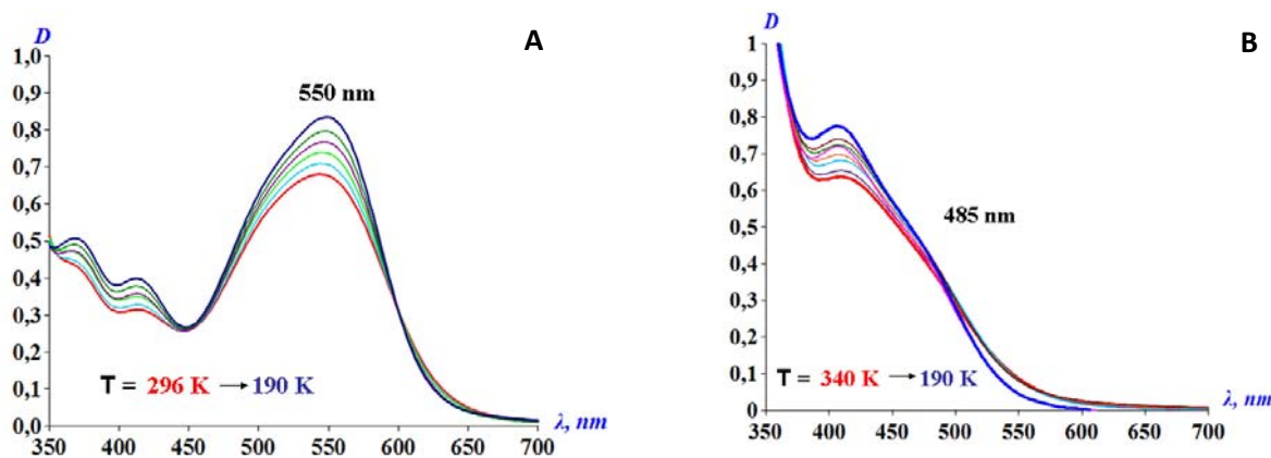
Figure 36. (A) UV-vis spectra of 4c ( c = 2.5 \cdot 10^{-3} M) in \text{CH}_2\text{Cl}_2 at 190 – 296 K (cell d = 0.22 cm). (B) UV-vis spectra of 3c ( c = 2.5 \cdot 10^{-3} M) in toluene at 190-340 K (cell d = 0.22 cm)
