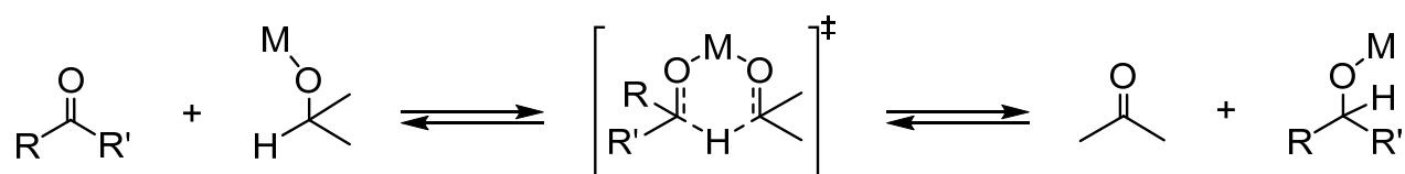
Scheme 10. The direct hydrogen transfer mechanism in the MPV reduction.
