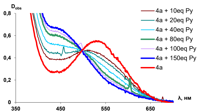
Figure 39. UV-vis titration of 4a ( c = 0.5 mM) with Py in \text{CH}_2\text{Cl}_2 , T = 296 K, cell d = 1 cm.
