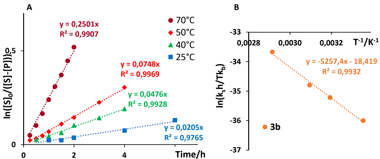
Figure 75. A) Kinetic curves for the formation of phenylethanol in i PrOH at different temperatures for complex 3b . B) Eyring analysis of the second order rate constant k . Reaction conditions as in Table 27.
