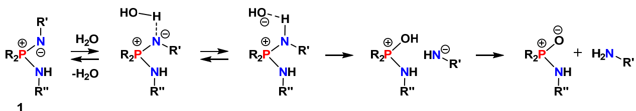
Scheme 22. Possible mechanism of hydrolysis 1 .
