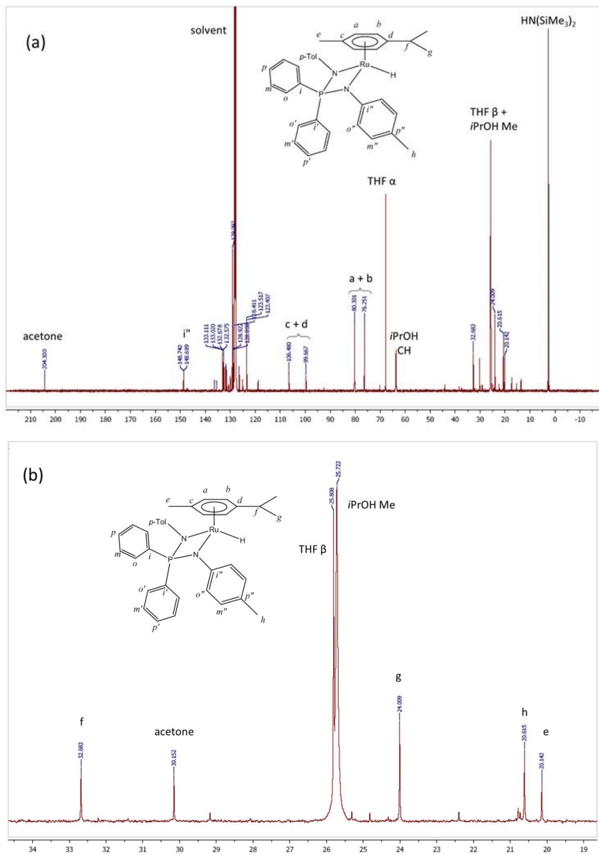
Figure S1. ^1\text{H} NMR spectra of 6f , generated in situ from 3f in \text{C}_6\text{D}_6 . Conditions: 0.5 mL of \text{C}_6\text{D}_6 , 13 mg of 3f (0.02 mmol), 60 \mu\text{L} of i\text{PrOH} ( i\text{PrOH}/1 = 40 ), 15 \mu\text{L} of NaHDMS (2M in THF; HMDS/ 3f = 1.5).
