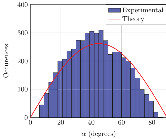
Figure 5.13 – Parameter distribution \alpha of 5000 channels constituted of n = 15 concatenated, randomly oriented, PDL elements of 1.1dB following the experimental setup in Fig. 5.11.
