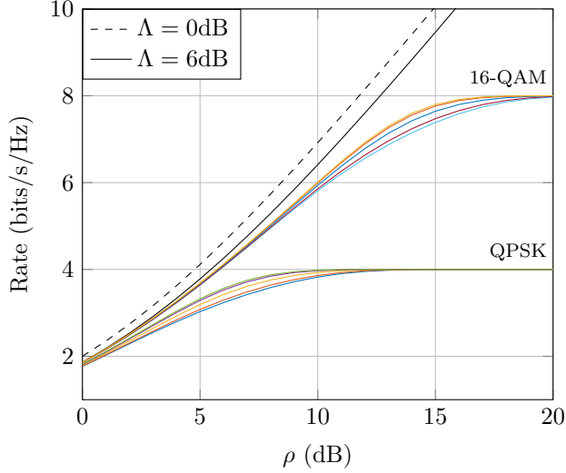
Figure 3.2 – DP- M -QAM rate function of the SNR for \Lambda = 6\text{dB} (full lines) and various SOPs for M = 4 and 16. The 2 \times 2 -MIMO capacity with no PDL (dashed line) is represented as a reference.
