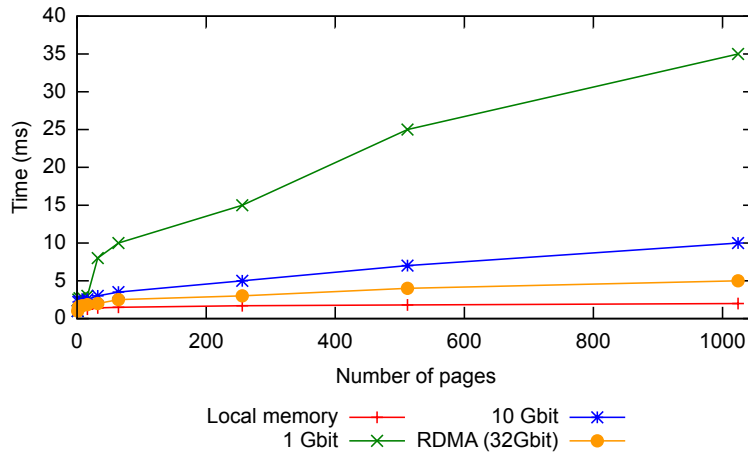
Figure 4.3: Latency while accessing pages in different locations
