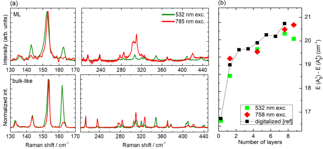
Figure 4.11: (a) Raman spectra for monolayer (top) and thick (bottom) flakes for different excitations wavelengths (b) \Delta E for 532 nm, 785 nm excitation and after [Qiao 2016].
