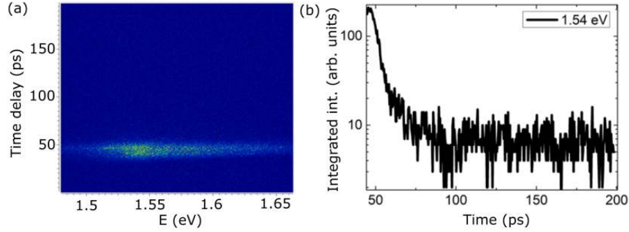
Figure 4.31: (a) Streak camera image of time-resolved PL emission measured at 10 K for a thick flake of \text{ReS}_2 . (b) Time profile profile showing the decay at 1.54 eV.
