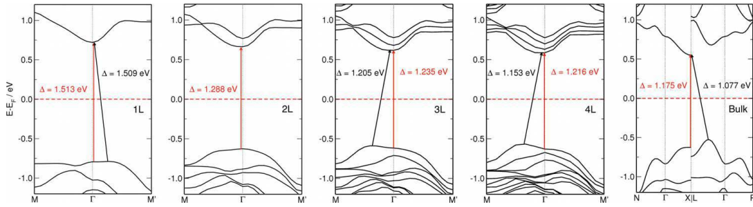
Figure 4.1: Calculated band structure for several layer \text{ReS}_2 . The red arrows mark the direct bandgap, the black arrows the fundamental bandgap. After [Urban 2019].
