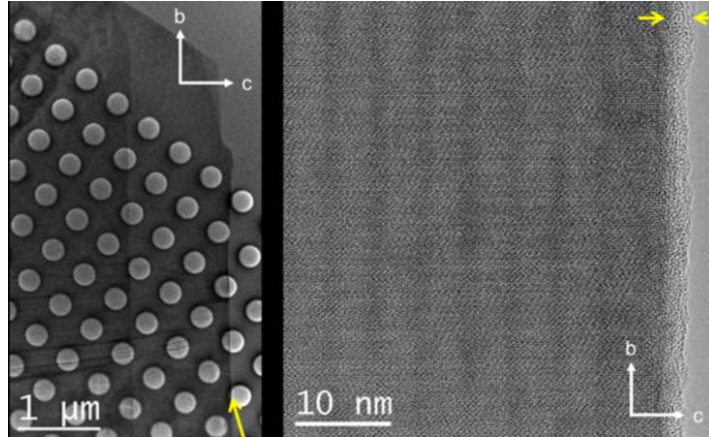
Figure 5.1: Optical microscopy image of a franckeite flake (left) placed on a TEM grid and TEM image (right) of a suspended part of the flake with clearly visible one-dimensional corrugation. The images were taken by our collaborators from the group of A. Castellanos-Gomez.
