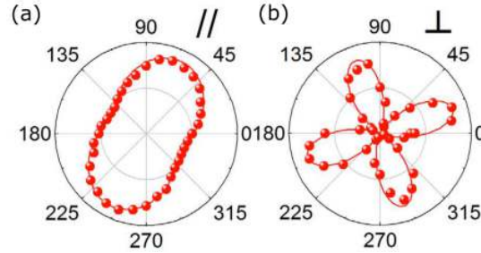
Figure 2.4: Polarization direction dependence of the Raman intensity for the 80 cm⁻¹ A_1 mode in \text{WTe}_2 in the (a) parallel and (b) perpendicular configuration. After [Song 2016b].
