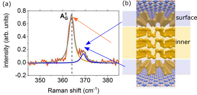
Figure 3.16: (a) Raman spectrum showing the high and low energy components of the A_g^1 mode and (b) schematics of the encapsulated BP crystal structure demonstrating the origin of the inner and surface modes observed in the spectrum.
