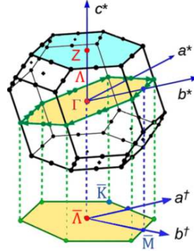
Figure 1.18: The Brillouin zone of ReS 2 . a^*, b^*, c^* are the reciprocal lattice vectors and the high-symmetry Z-plane, \Gamma -plane and its projection on the k_z =constant plane are shaded [Webb 2017].
