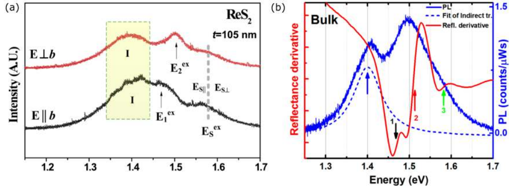
Figure 1.16: (a) \mu -PL spectra for two different polarizations for thick \text{ReS}_2 with marked indirect transition (I), two lowest direct transitions E_1^{\text{ex}} and E_2^{\text{ex}} and a higher energetic excitonic transition E_S^{\text{ex}} . After [Ho 2017]. (b) Photoluminescence (blue) and a derivative of the reflectance (red) spectrum. Arrows indicate the positions of optical transitions. After [Aslan 2016].
