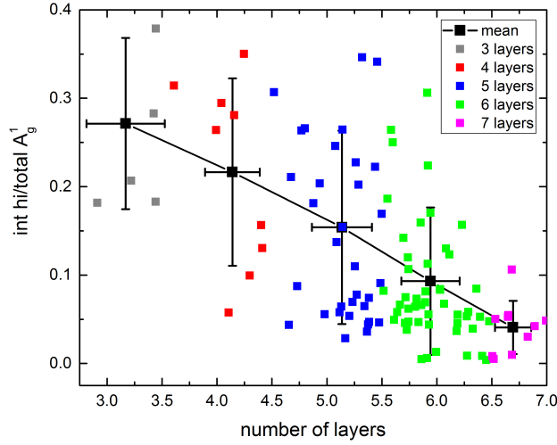
Figure 3.14: Intensity ratio of the high energy peak to the total intensity (sum of the high- and low-energy component intensities) for the A_g^1 mode as a function of the number of layers. The black points with error bars show mean values for each number of layers.
