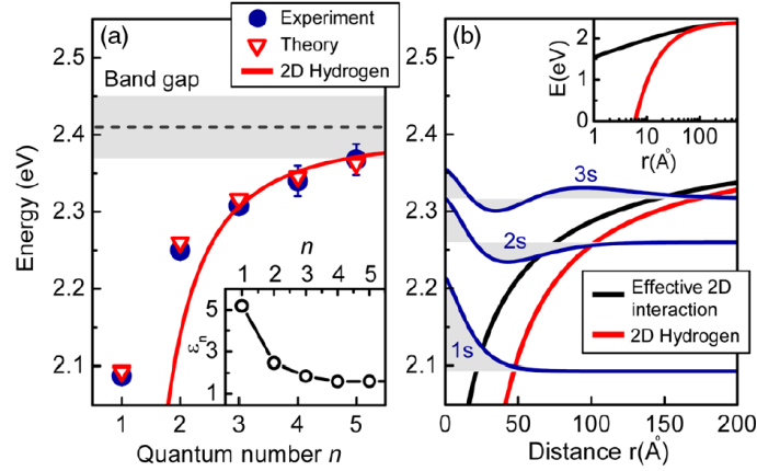
Figure 1.3: (a) Energies of the ground and excited exciton states in ML WS 2 determined experimentally and calculated theoretically, together with a fit of the 2D hydrogen model to the three highest states. The inset shows the effective dielectric constant. (b) Comparison of the nonlocal screening interaction potential (black) and the 2D hydrogen model (red) and the radial wave functions for the lowest excitonic states (blue). The inset shows the same dependence in semilogarithmic scale. After [Chernikov 2014].
