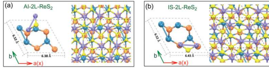
Figure 1.14: Schematic of the (a) AI-stacked and (b) IS-stacked bilayer \text{ReS}_2 . After [Qiao 2016].
