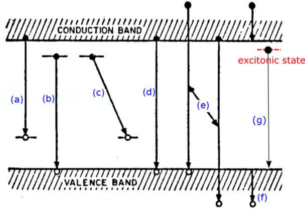
Figure 2.1: Luminescence recombination processes in a semiconductor: (a) conduction band to acceptor, (b) donor to valence band, (c) donor to acceptor, (d) band edge emission, (e) hot PL emission, (f) intraband relaxation processes, (g) recombination from an excitonic state. Adapted from [Dresselhaus 2018].
