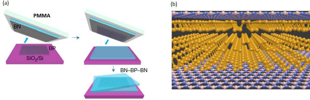
Figure 3.4: (a) Schematic of the encapsulated sample fabrication process, after [Chen 2015] and (b) crystal structure of BP encapsulated in h-BN.
