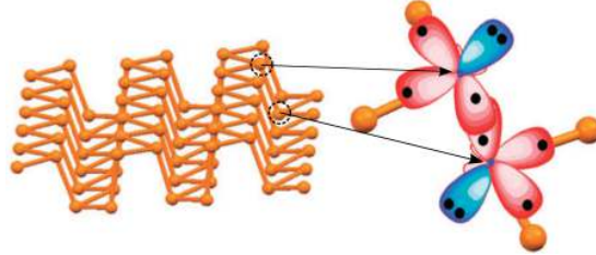
Figure 1.5: Atomic structure of monolayer BP and sketch of the hybridization of the orbitals. Red indicates \sigma orbitals and blue the lone electron pairs. Adapted from [Boukhalov 2015].
