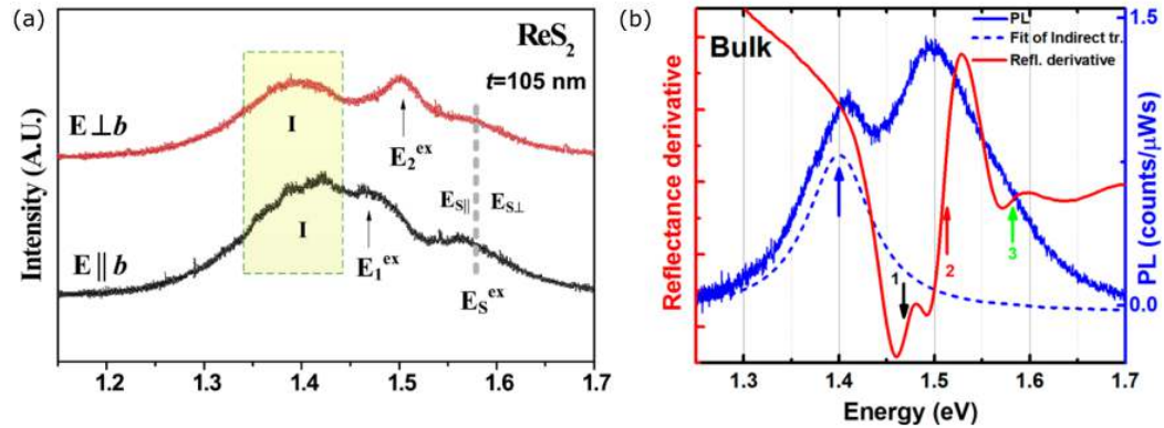
Figure 1.16: (a) \mu -PL spectra for two different polarizations for thick ReS 2 with marked indirect transition (I), two lowest direct transitions E_1^{ex} and E_2^{ex} and a higher energetic excitonic transition E_S^{ex} . After [Ho 2017]. (b) Photoluminescence (blue) and a derivative of the reflectance (red) spectrum. Arrows indicate the positions of optical transitions. After [Aslan 2016].
