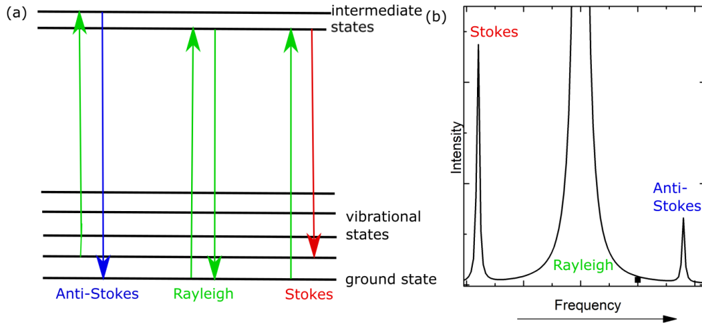
Figure 2.2: (a) The schematics of the energy levels in elastic and inelastic scattering processes. The arrows mark the incoming and scattered photons. (b) Schematics of a Raman spectrum showing the Stokes and anti-Stokes lines and the Rayleigh elastically scattered line.
