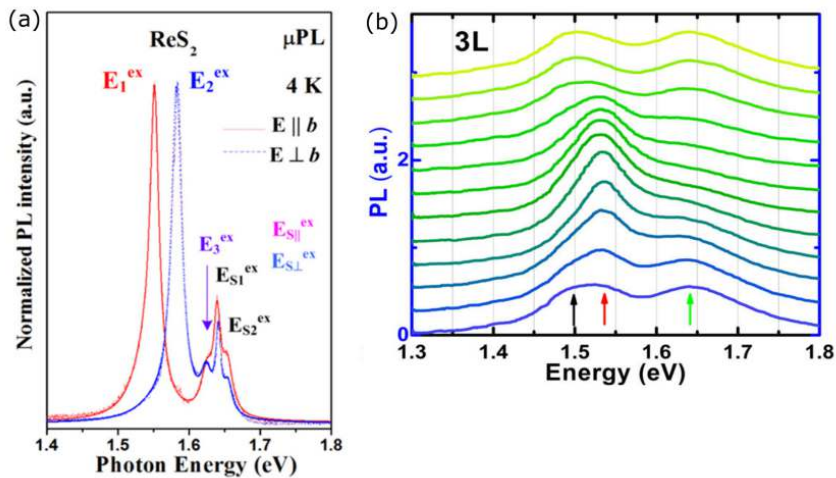
Figure 1.17: (a) Polarized PL spectra of few layer thick ReS 2 for detection polarization parallel (red) and perpendicular (blue) to the rhenium chains. After [Ho 2019]. (b) Polarization-resolved photoluminescence spectra measured at 15° intervals. After [Aslan 2016].
