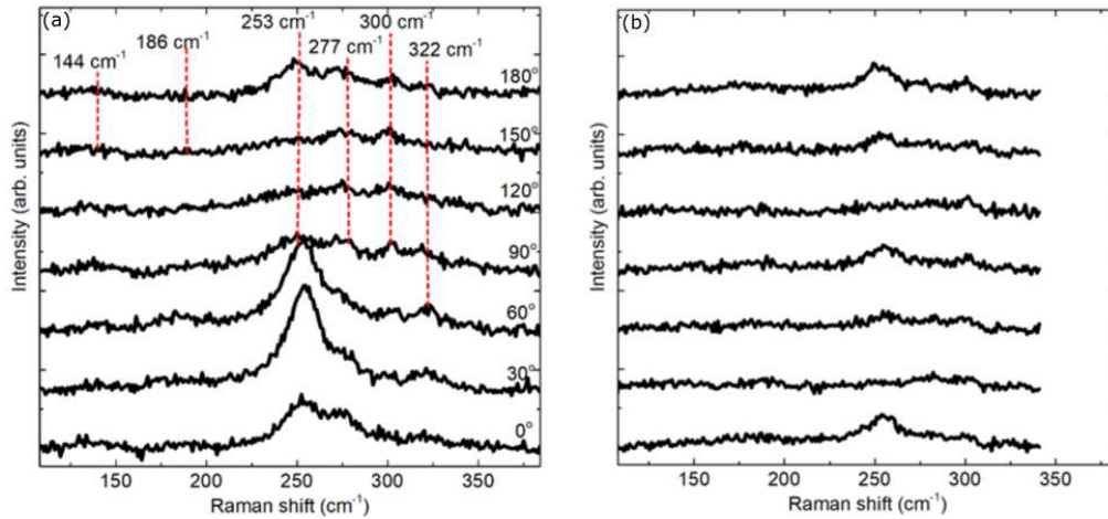
Figure 5.12: Chosen Raman spectra for different excitation angles at 30^\circ intervals for the (a) co- and (b) cross-polarization configurations.
