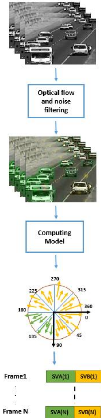
Figure 23: The different steps for normal traffic modeling 51
