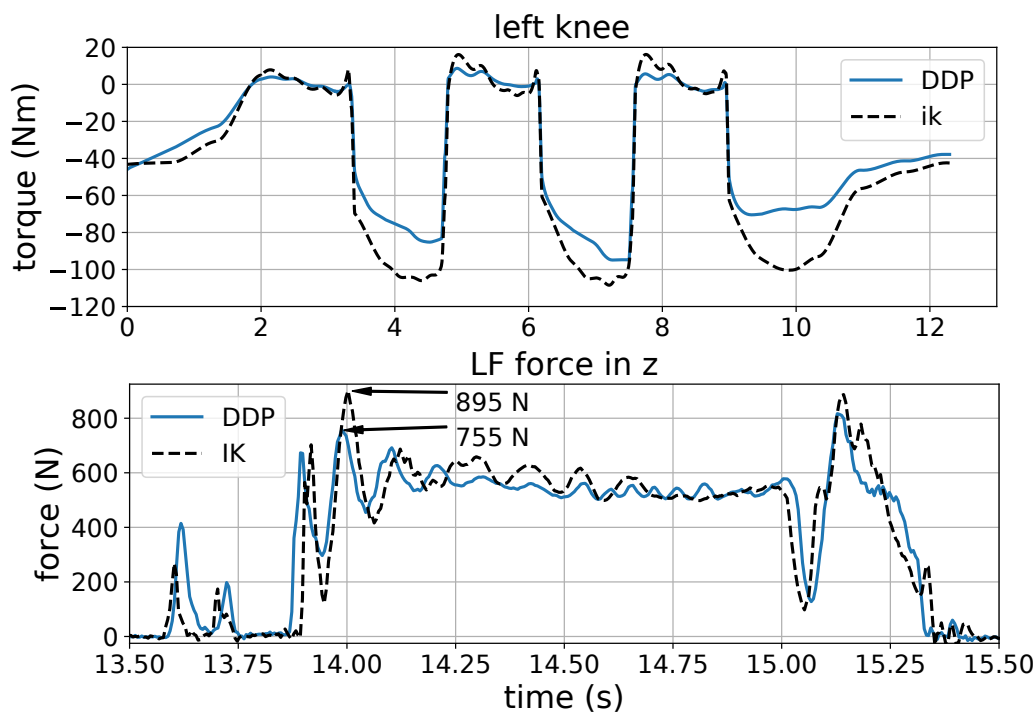
Fig. 3.4: Comparison between the IK and DDP trajectory for 100 cm stride on the HRP-2 robot. Top: Knee torques generated in the left leg. Bottom: Ground Reaction Forces (GRFs) generated in the left foot. The DDP formulation allows us to utilize the angular momentum of the upper body, which reduces the requirement on the lower body to create a counterbalancing motion. This results in a lower torque in the lower body, as well as lower GRFs. Around t = 14s we can see high peaks for the IK and DDP trajectories of 895 N and 755 N, respectively.
