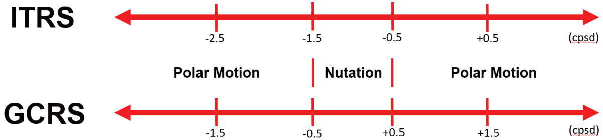
Figure A.4 – Frequency division of nutation and polar motion in the terrestrial and celestial frequency band. The frequency unit is cycle per siderial days (cpsd). This image is based on IERS Convention 2010.
