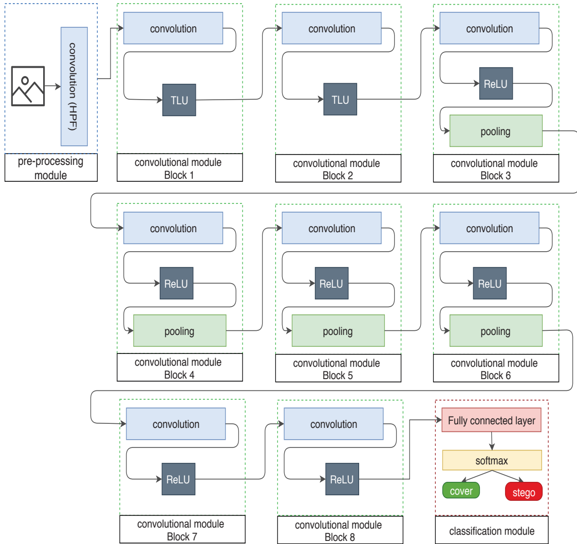
FIGURE 5.8: Ye-Net overall architecture.
