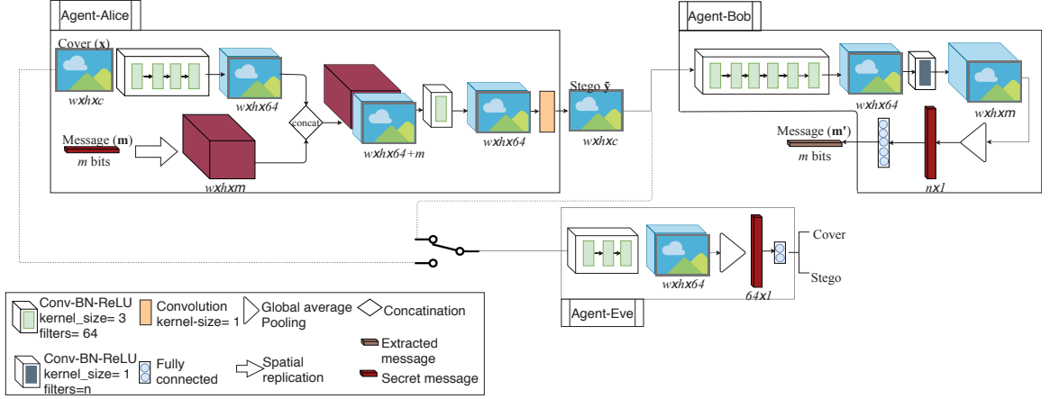
FIGURE 8.2: HiDDeN architecture.
