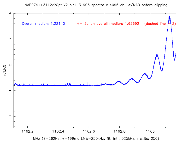
FIGURE 4.33: B0738+313: \frac{\sigma}{MAD} before clipping within the 1162.11 - 1163.18 MHz Local Standard of Rest (LSR) frequency band.
