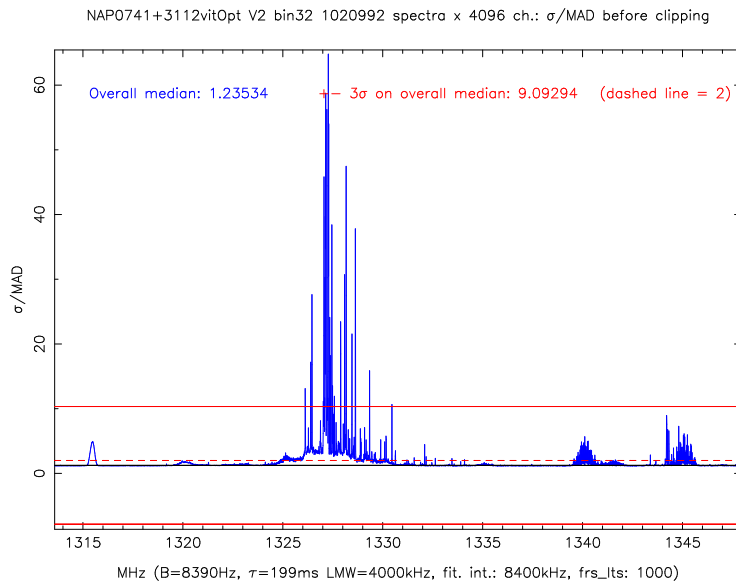
FIGURE 4.53: RN radar: \frac{\sigma}{\text{MAD}} for the ON unclipped spectrum in the 1324 – 1332 MHz frequency band (robust binning 32 times).
