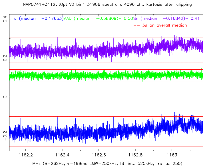
FIGURE 4.40: B0738+313: kurtosis after \sigma -clipping (blue line), MAD-clipping (green line), and Sn-clipping (purple line) within the 1162.11 - 1163.18 MHz Local Standard of Rest (LSR) frequency band.
