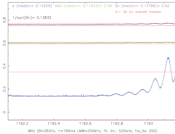
FIGURE 4.34: B0738+313: normalized estimators of scale before clipping within the 1162.11 - 1163.18 MHz Local Standard of Rest (LSR) frequency band.
