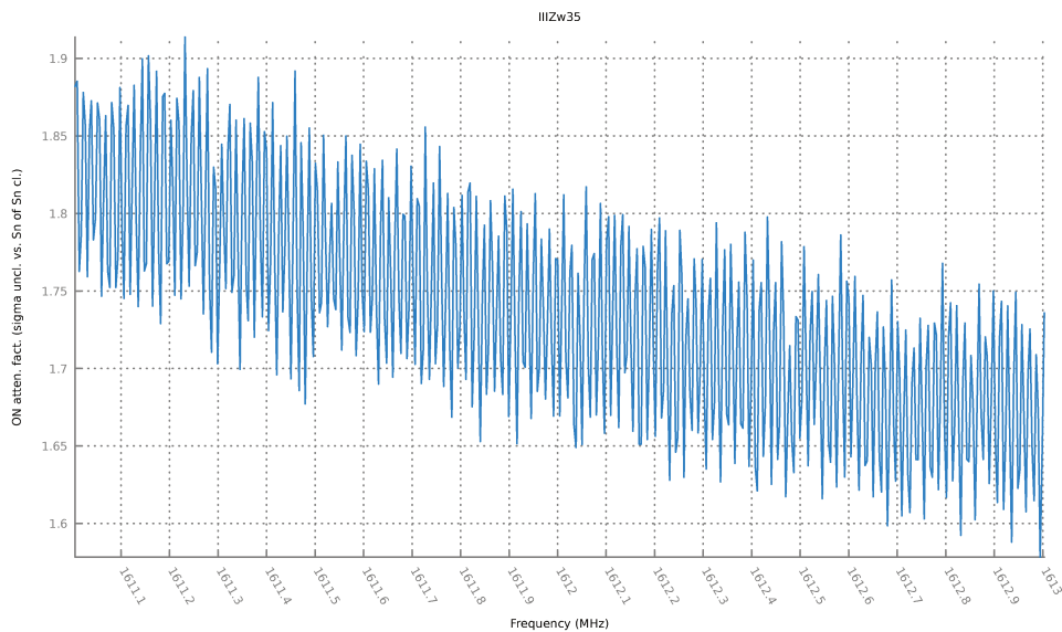
FIGURE 4.73: Temporal EoS (estimator of scale) attenuation factor ( S_n of S_n -clipped median - \sigma of unclipped median) / ( S_n of S_n -clipped median) of uncalibrated averaged power spectral values of the ON spectrum in the 1611 – 1613 MHz protected frequency band.
