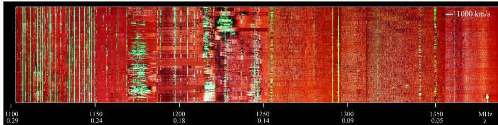
FIGURE 1.1: Broadband spectrum observed at the Nançay decimetric radio telescope (NRT) with the standard autocorrelator in 2011 (van Driel & Lehnert, private communication). Shown in this so-called waterfall diagram are one-hour long time series of ON - OFF power spectra. Indicated along the horizontal axis are frequencies (from 1100 to 1380 MHz) and the corresponding redshifts z of the 21 cm HI line (from 0.03 to 0.29); the horizontal white bar indicates a radial velocity range of 1000 \text{ km s}^{-1} . RFI flagged by the standard NRT data reduction package (see Monnier Ragaigine et al. (2003)) is shown in green whereas the sky background is shown in red.
