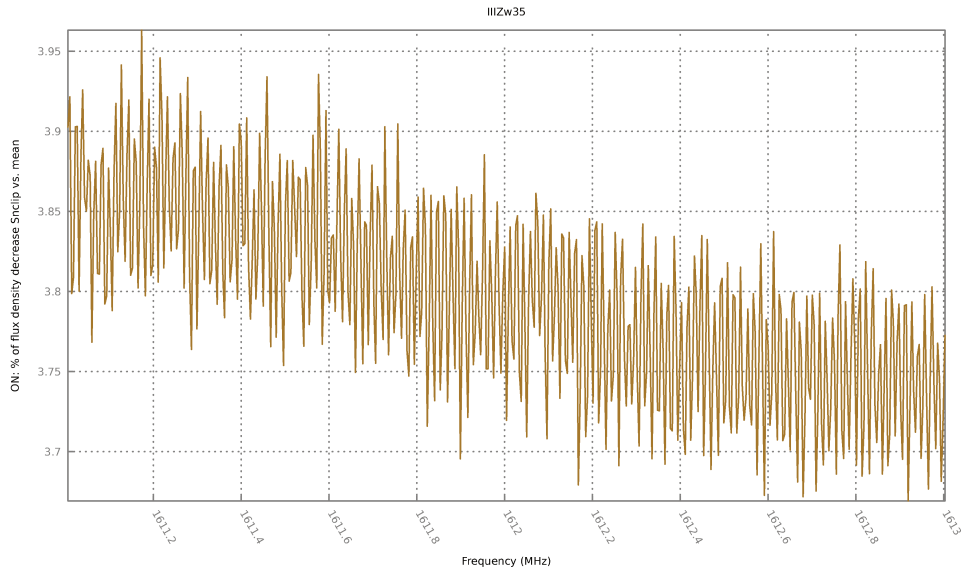
FIGURE 4.72: EoL attenuation factor (unclipped mean - S_n -clipped median) / ( S_n -clipped median) of uncalibrated averaged power spectral values of the ON spectrum in the 1611 – 1613 MHz protected frequency band.
