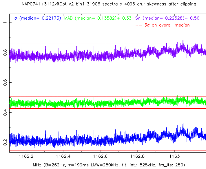
FIGURE 4.39: B0738+313: skewness after \sigma -clipping (blue line), MAD-clipping (green line), and Sn-clipping (purple line) within the 1162.11 - 1163.18 MHz Local Standard of Rest (LSR) frequency band.
