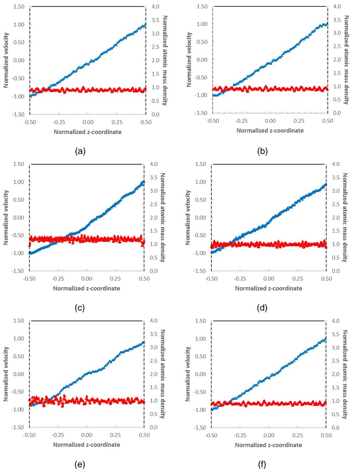
Figure IV.5. Velocity (blue) and atomic mass density (red) profiles for benzyl benzoate at 313 K, 50 \text{ m.s}^{-1} , and (a) 0.5 GPa and (b) 2 GPa, squalane at 50 \text{ m.s}^{-1} , (c) 353 K and 2 GPa, and (d) 313 K and 1.2 GPa, and finally the NPE mixture at 50 \text{ m.s}^{-1} , 300K, and (e) 0.8 GPa and (f) 1.4 GPa. The velocity profile has been normalized with respect to the imposed sliding wall velocity, and the density profile with respect to the bulk density value at the given pressure and temperature conditions. They are represented versus the normalized z-
