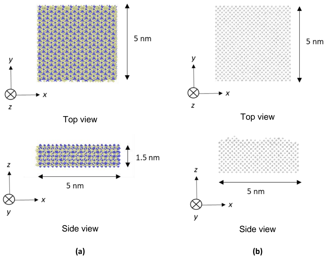
Figure II.5. Examples of surfaces used for the confined simulations: (a) atomsically smooth iron oxide and (b) randomly rough iron surfaces. In (a), yellow particles are O atoms and blue particles are Fe atoms.
