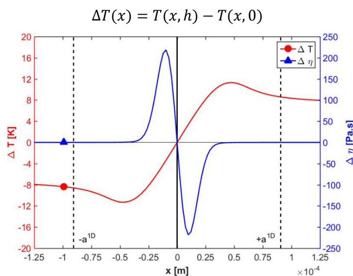
Figure 3.1-2 – Temperature and viscosity differences between the two interfaces at 2 \text{ m.s}^{-1} . The vertical lines mark the location of a^{1D} .
