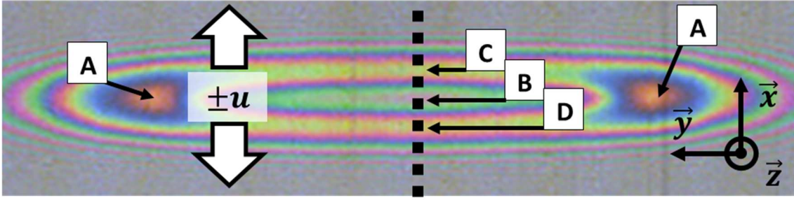
Figure 2.2-4 – Interferogram obtained with a sapphire disc (Magnification \times 10 , u = 5 \text{ m/s} , w^{2D} = 50 \text{ N} and T_0 = 293.15 \text{ K} ).
