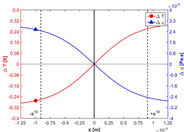
Figure D-2 – Temperature and viscosity differences between the two interfaces at 3 \text{ m} \cdot \text{s}^{-1} and w^{1D} = 67 \text{ N} \cdot \text{m}^{-1} .
