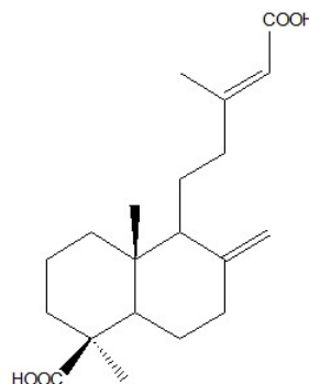
Figure 20: Acide agathique.
