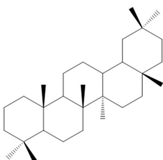
Figure 26: Oléanane.
