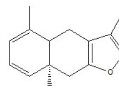
Figure 36: Furanoedesma-1,3- diène.
