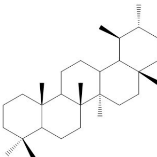
Figure 27: Ursane.
