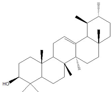
Figure 32: \alpha -amyrine.
