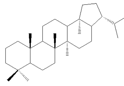
Figure 31: Hopane.
