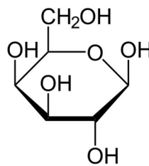
Figure 50: Galactose.
