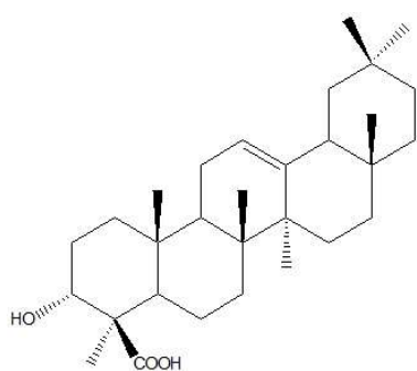
Figure 34: \alpha -boswellique.
