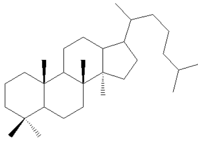
Figure 30: Dammarane.
