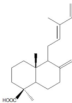
Figure 19: Acide commune.
