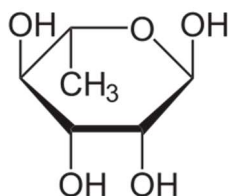
Figure 51: Rhamnose.
