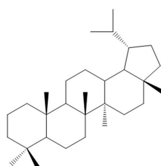
Figure 28: Lupane.
