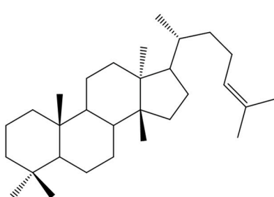
Figure 29: Euphane.
