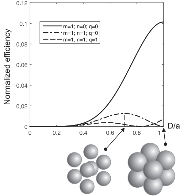
Figure 2.9: Normalized efficiency of SC lattice for three first orders (1, 0, 0) , (1, 1, 0) , and (1, 1, 1) as a function of ratio between the spherical motif diameter, D , and the lattice periodicity, a . Normalized efficiency is calculated for the “+/-” structure.
