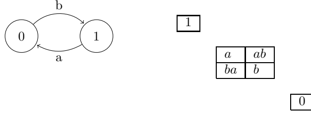
Figure 5.8: Automaton that generates the monoid M = \{\varepsilon, a, b\} .
