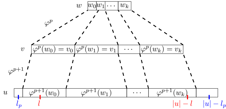
Figure 3.13: A graphical explanation of the proof of Theorem 3.4.1.
